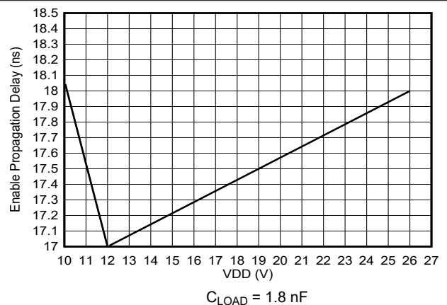
Figure 5-20. Enable to Output Rising Propagation Delay
