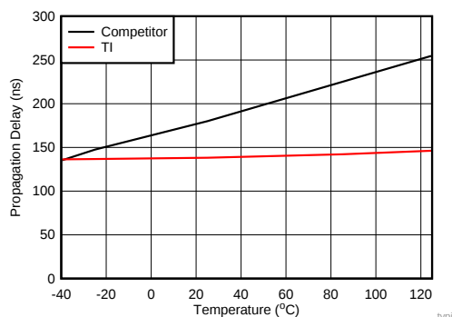
Typical Propagation Delay Comparison
