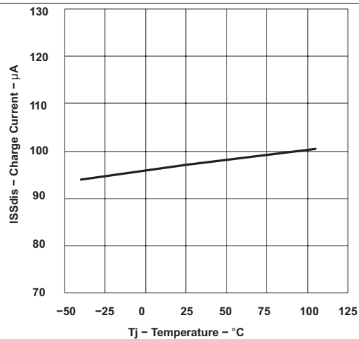
Figure 12. Soft-Start Discharge Current vs Temperature
