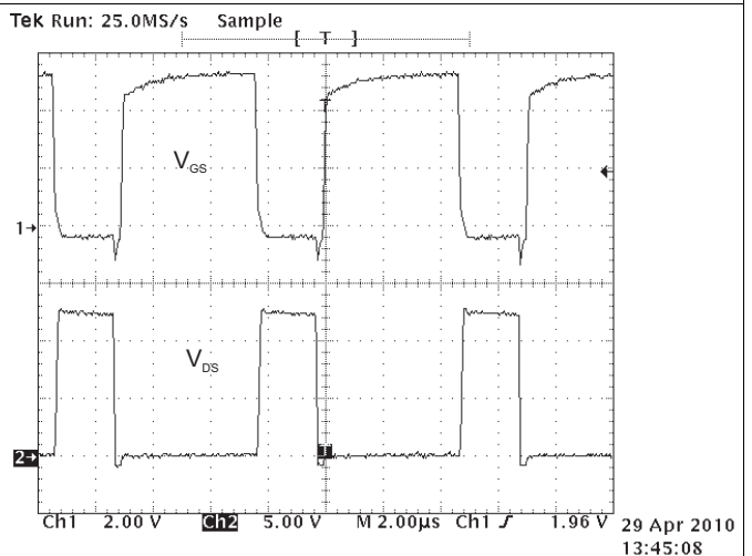
Figure 52. Secondary-Side Switching Waveform
