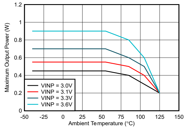
Figure 6-4. Maximum Output Power vs Ambient Temperature : VCC = 5.0V , COUT2 = 22µF
