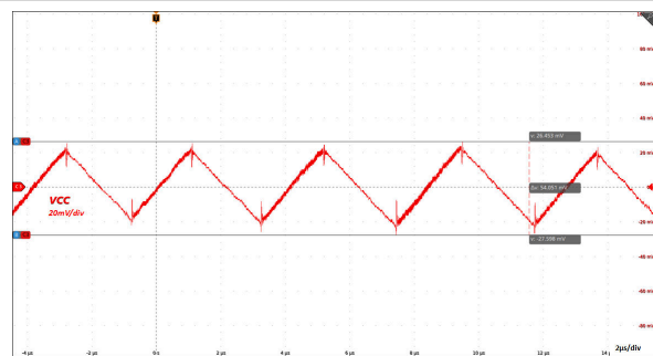
Figure 8-3. Steady State Output Voltage Ripple: VINP = 5.0V, VCC = 5.0V , C OUT2 = 22μF, 300mA Load
