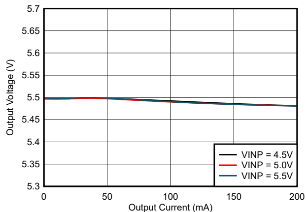
Figure 6-12. Output Voltage Regulation ( V_{VCC} ) vs Load Current ( I_{VCC} ): V_{CC} = 5.5V , T_A = 25^\circ C , C_{OUT2} = 22\mu F
