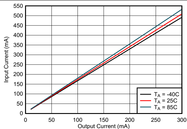
Figure 6-9. Input Current ( I_{VINP} ) vs Load Current ( I_{VCC} ): V_{CC} = 5.0V , V_{INP} = 5.0V , C_{OUT2} = 22\mu F
