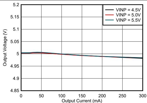
Figure 6-10. Output Voltage Regulation ( V_{VCC} ) vs Load Current ( I_{VCC} ): V_{CC} = 5.0V , T_A = 25^\circ C , C_{OUT2} = 22\mu F
