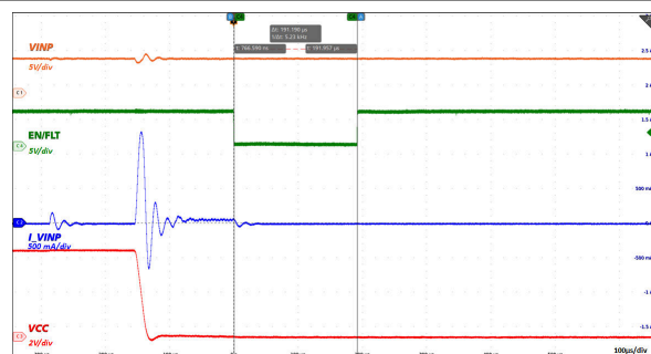
Figure 6-16. Output Short Circuit Operation: VINP = 5.0V
