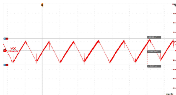
Figure 6-14. Steady State Output Voltage Ripple: VINP = 5.0V, VCC = 5.0V, 300mA Load
