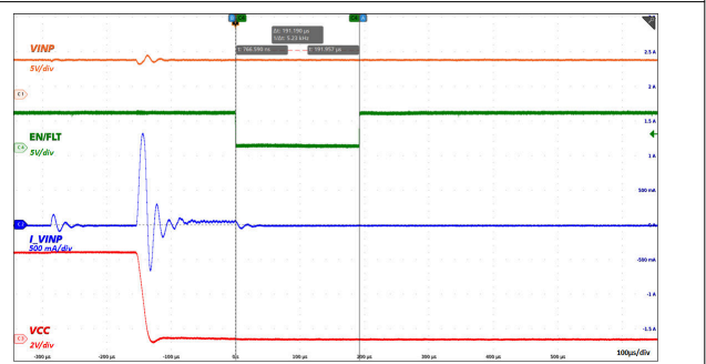
Figure 8-5. Output Short Circuit Operation: VINP = 5.0V
