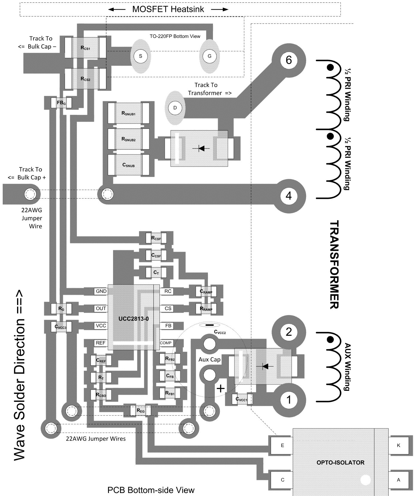
Figure 8-12. UCC2813-0 Layout Example for Single-Layer PCB
