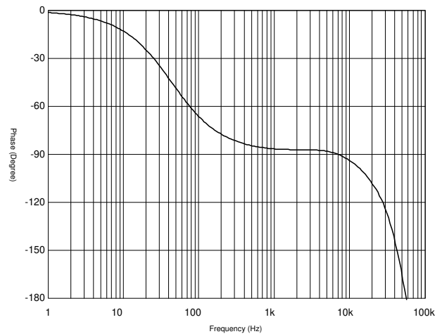
Figure 8-3. Converter Open-Loop Bode Plot: Phase
