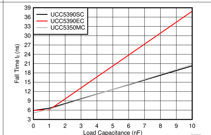
Figure 6-40. Fall Time vs Load Capacitance
