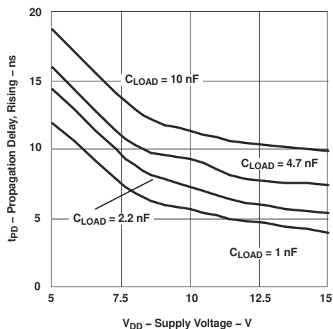
Figure 8-9. Propagation Delay Rising vs Supply Voltage
