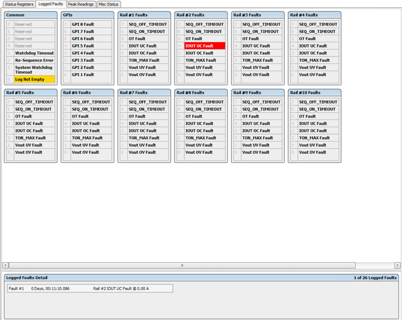
Figure 7-5. Fusion GUI Flash-Error Log (Logged Faults)
