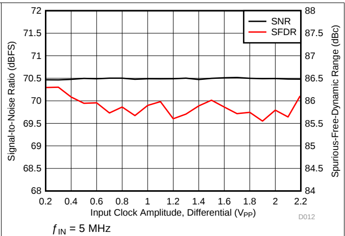
Figure 15. Performance vs Input Clock Amplitude
