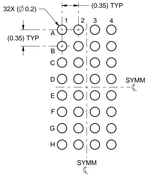
LAND PATTERN EXAMPLE SCALE:20X
