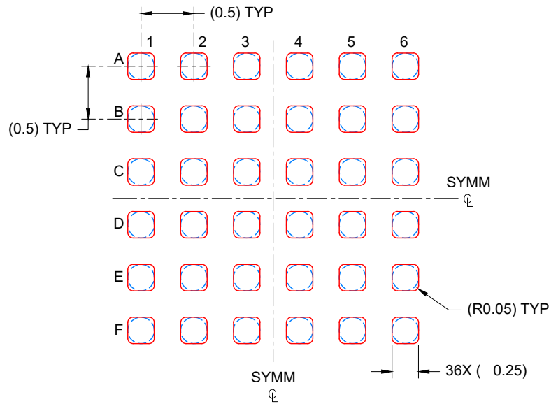
SOLDER PASTE EXAMPLE BASED ON 0.100 mm THICK STENCIL SCALE: 20X
