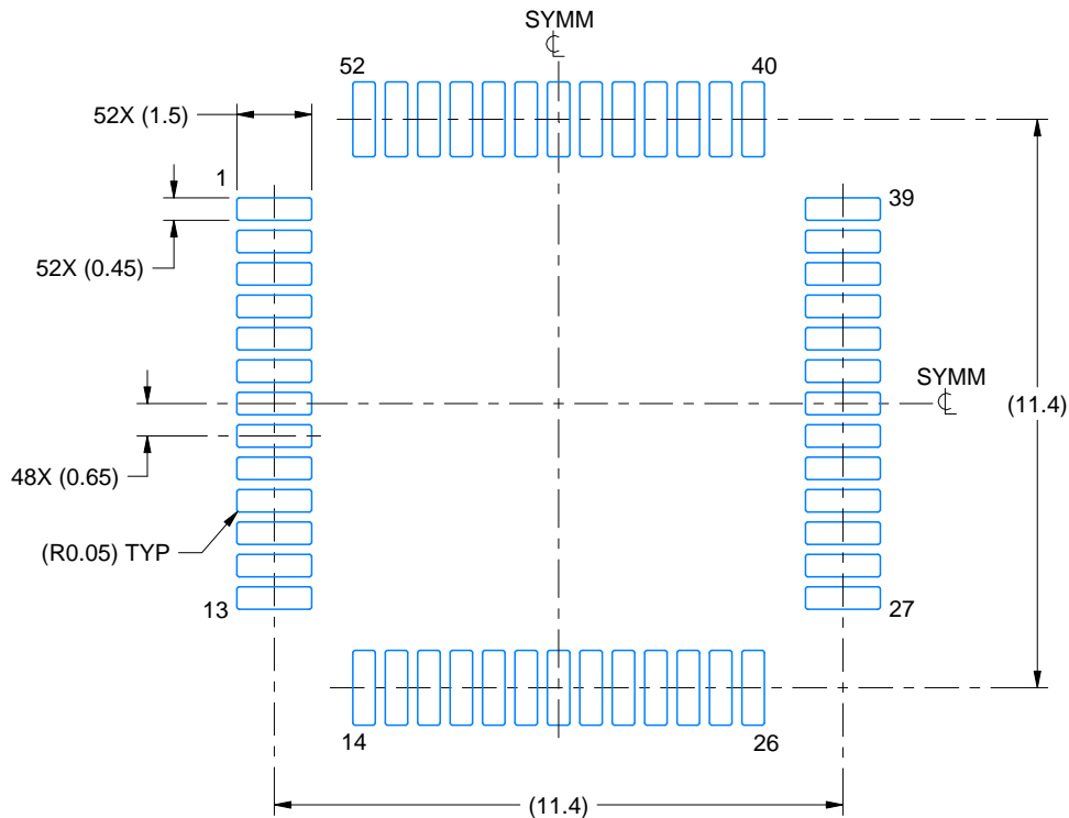
LAND PATTERN EXAMPLE EXPOSED METAL SHOWN SCALE:6X
