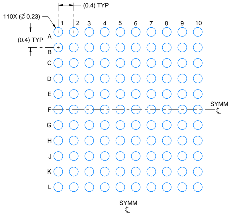
LAND PATTERN EXAMPLE EXPOSED METAL SHOWN SCALE:18X
