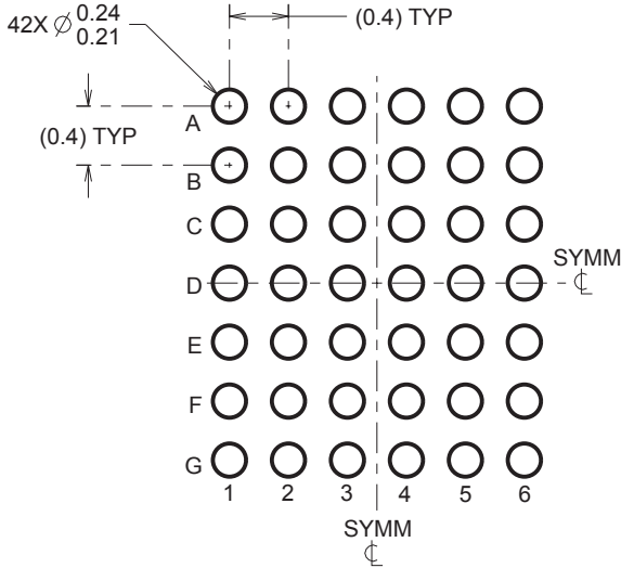
LAND PATTERN EXAMPLE SCALE:18X
