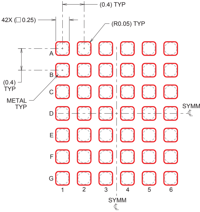
SOLDERPASTE EXAMPLE BASED ON 0.1mm THICK STENCIL SCALE:25X
