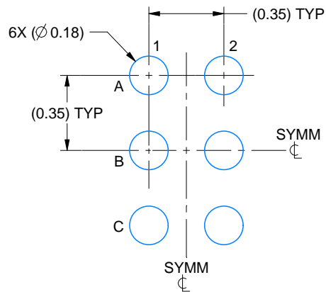
LAND PATTERN EXAMPLE SCALE:40X
