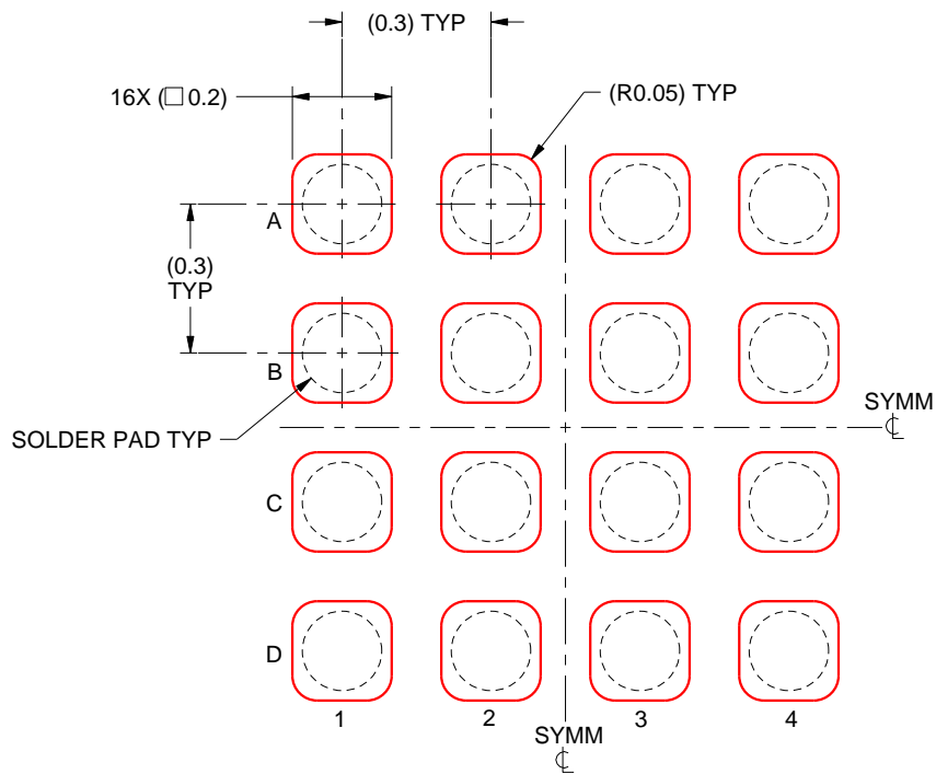
SOLDER PASTE EXAMPLE BASED ON 0.075 mm THICK STENCIL SCALE:60X
