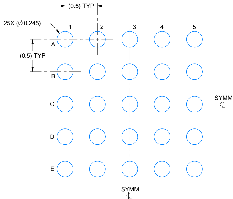
LAND PATTERN EXAMPLE EXPOSED METAL SHOWN SCALE:30X
