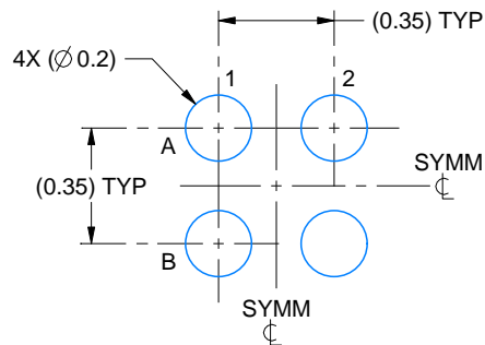
LAND PATTERN EXAMPLE SCALE:40X
