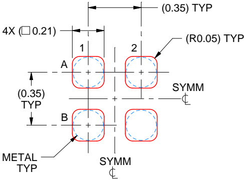
SOLDER PASTE EXAMPLE BASED ON 0.075 - 0.1 mm THICK STENCIL SCALE:40X
