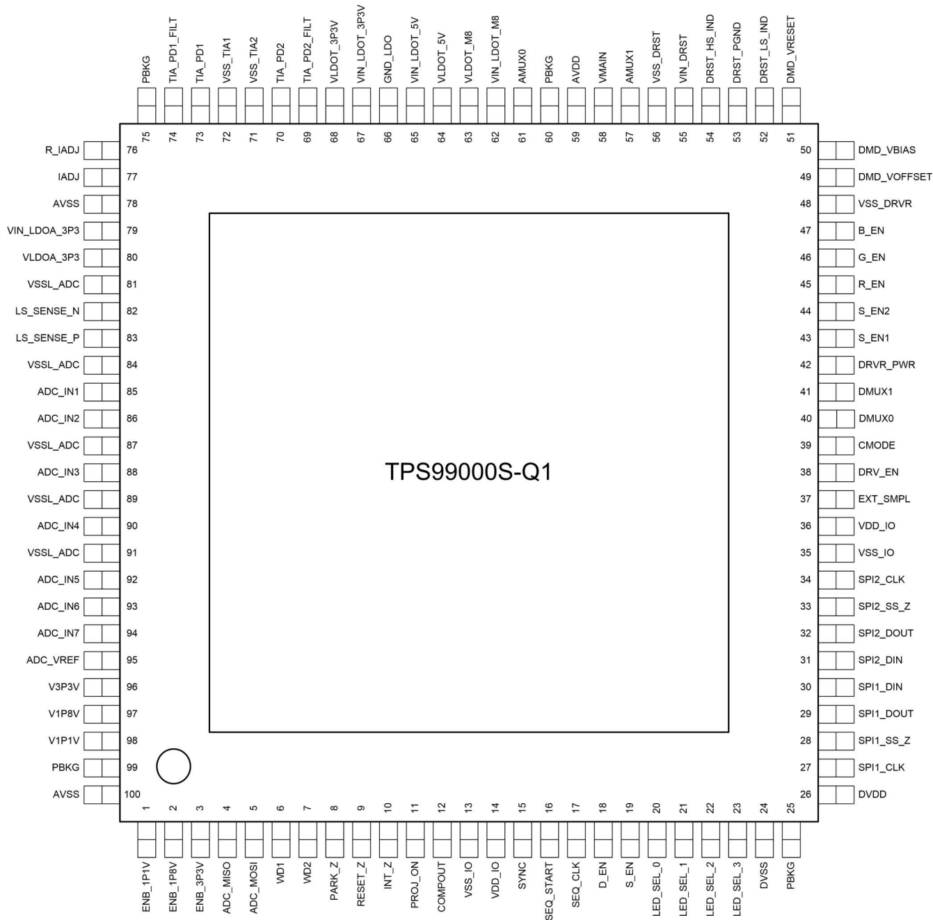
Figure 4-1. PZP Package 100-Pin HTQFP Top View
