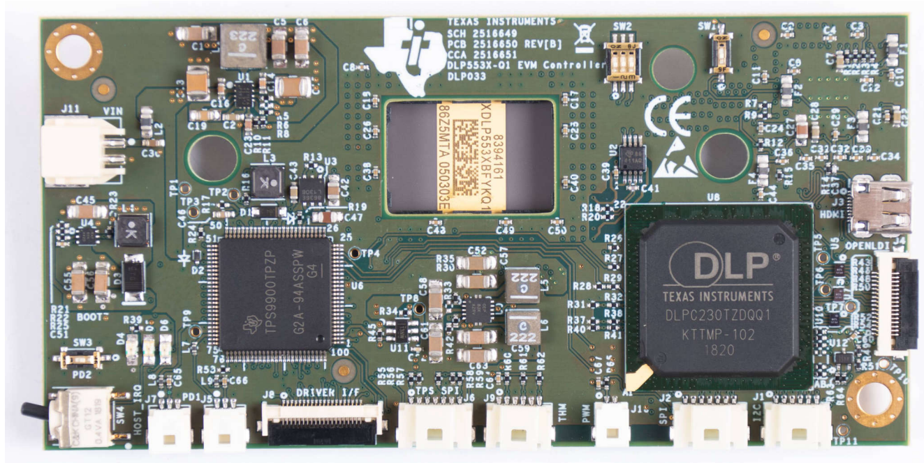
Figure 1-1. DLP5530PROJTGQ1EVM Controller PCB
