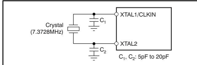
Figure 47. Crystal Connection
