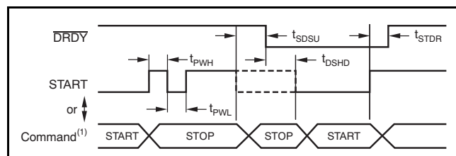
Figure 50. START to DRDY Timing
