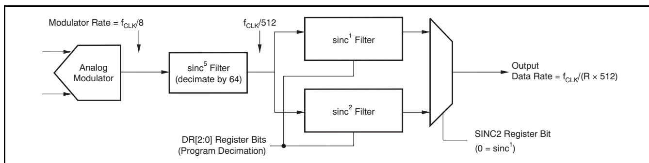
Figure 39. Block Diagram of Digital Filter
