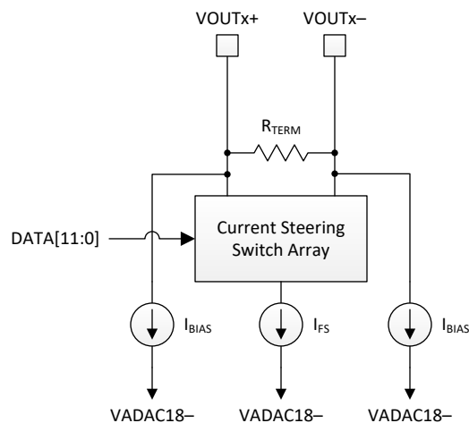
Figure 7-9. DAC12DL3200 Analog Output Structure
