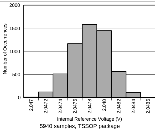
Figure 24. Internal Reference Voltage Histogram
