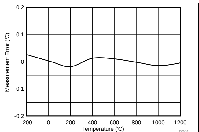
Figure 78. Temperature Measurement Error vs T_{(\text{TC})}
