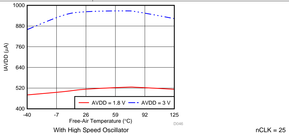
Figure 38. I_{AVDD} in High Precision Mode with Temperature
