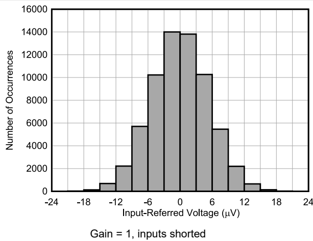
Figure 6-20. Single Device Noise Histogram at 4 kSPS
