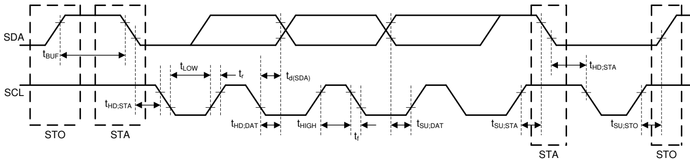
Figure 1. I²C Interface Timing Diagram
