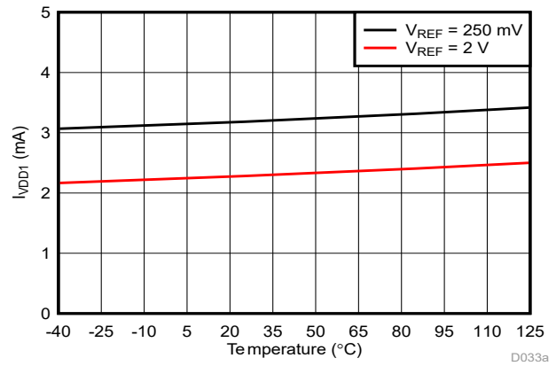
Figure 5-61. High-Side Supply Current vs Temperature
