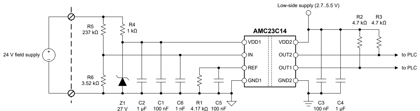
Figure 7-2. Using the AMC23C14 for Overvoltage and Undervoltage Detection
