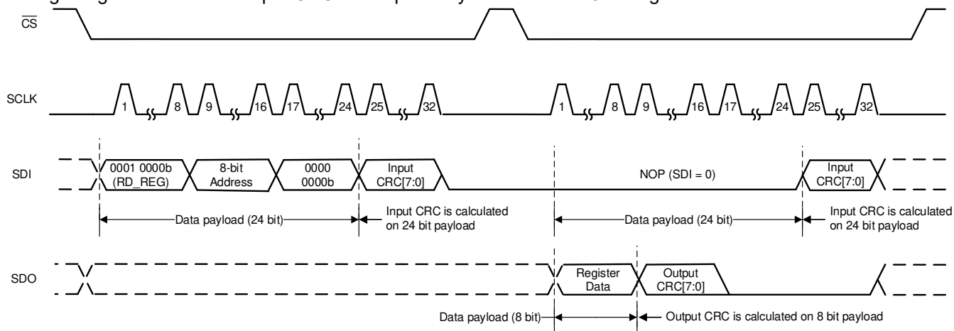
Figure 8-13. Register Read With CRC
