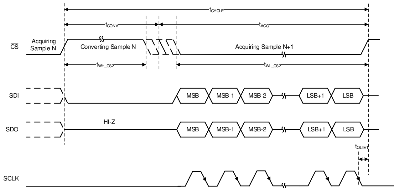
Figure 7-1. Conversion Cycle Timing
