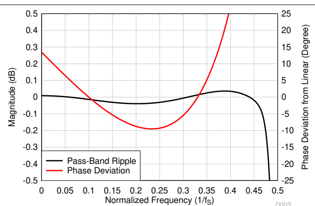
Figure 8-54. Ultra-Low-Latency Decimation Filter Pass-Band Ripple and Phase Deviation
