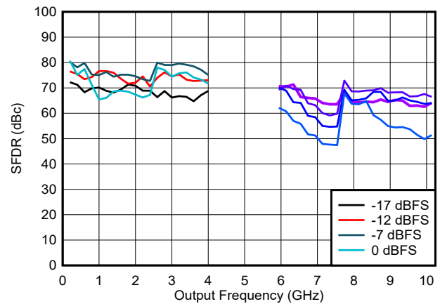
Figure 6-104. SFDR vs Frequency and Digital Amplitude in NRZ/RF Modes
