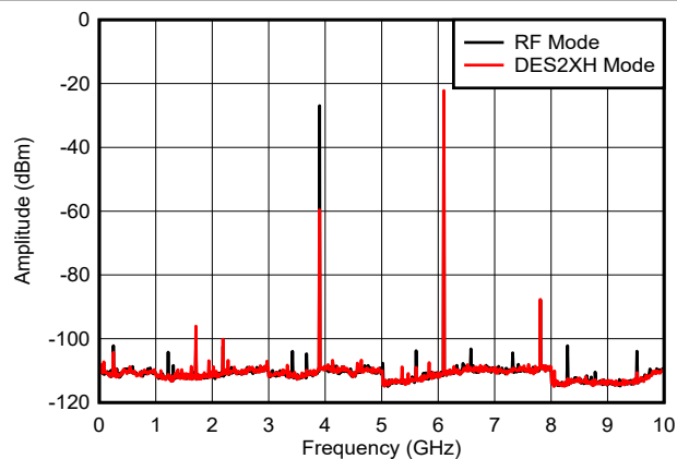
includes PCB, cable and balun loss Figure 6-33. f_{\text{OUT}} = 6097\text{ MHz} , -12 dBFS
