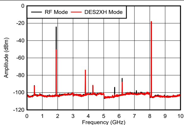
includes PCB, cable and balun loss Figure 6-35. f_{\text{OUT}} = 8097\text{ MHz} , -6 dBFS
