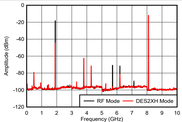
includes PCB, cable and balun loss Figure 6-34. f_{\text{OUT}} = 8097\text{ MHz} , 0 dBFS
