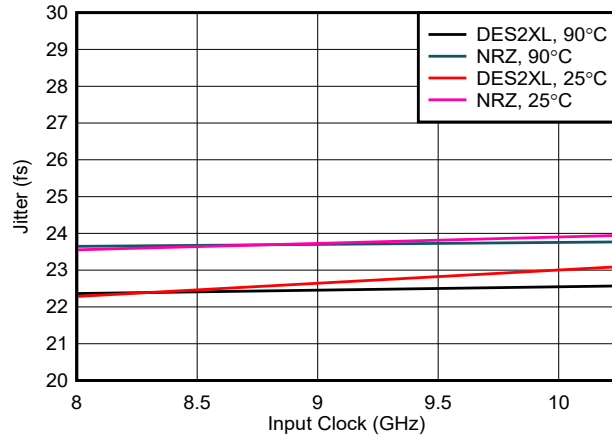
Figure 6-207. Jitter vs Input Clock
