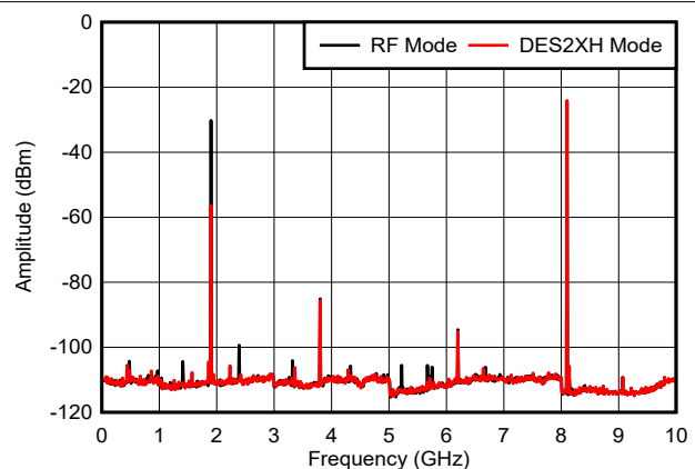
includes PCB, cable and balun loss Figure 6-36. f_{\text{OUT}} = 8097\text{ MHz} , -12 dBFS
