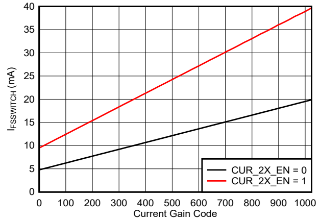
Figure 6-15. I_{\text{FS\_SWITCH}} vs Gain Code
