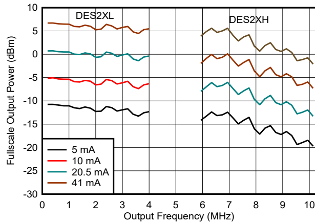
Figure 6-10. Output Power vs Frequency (DES2X modes)
