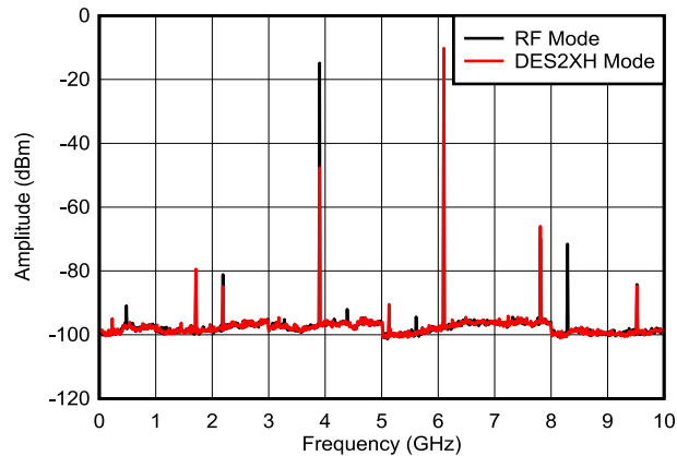
includes PCB, cable and balun loss Figure 6-31. f_{\text{OUT}} = 6097\text{ MHz} , 0 dBFS
