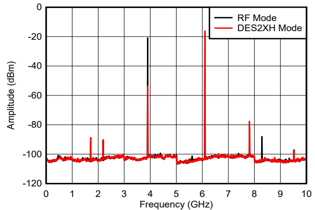
includes PCB, cable and balun loss Figure 6-32. f_{\text{OUT}} = 6097\text{ MHz} , -6 dBFS
