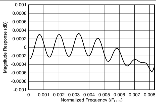
Figure 7-33. 48x Interpolation Filter Passband Response
