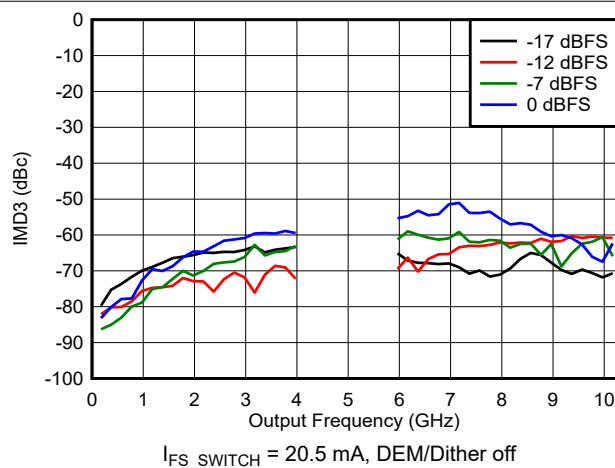
Figure 6-121. IMD3 vs Frequency and Digital Amplitude in DES2X Modes
