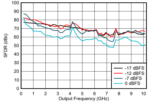
Figure 6-102. SFDR vs Frequency and Digital Amplitude in NRZ/RF Modes
