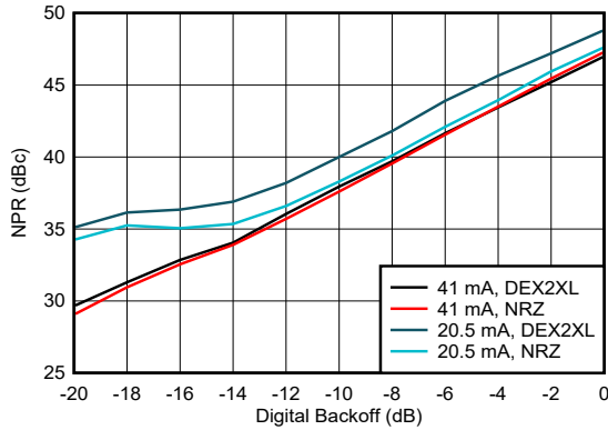
Figure 6-195. Noise Power Ratio vs Digital Backoff: 1 st Nyquist Zone
