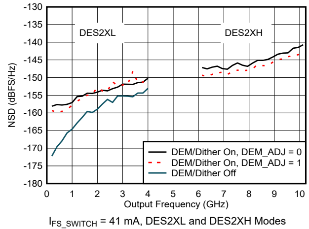
Figure 6-59. NSD vs Output Frequency and DEM/Dither Mode
