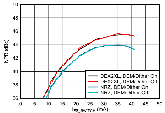
Figure 6-200. Noise Power Ratio vs Output Current: 2 nd Nyquist Zone
