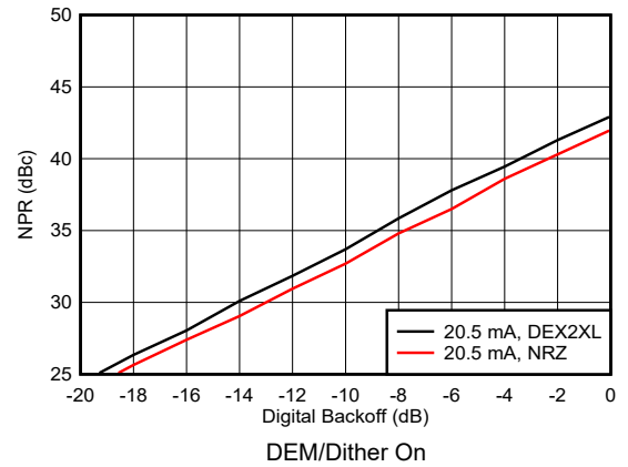
Figure 6-198. Noise Power Ratio vs Digital Backoff: 2 nd Nyquist Zone
