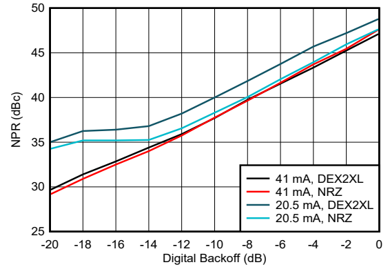
Figure 6-196. Noise Power Ratio vs Digital Backoff: 1 st Nyquist Zone
