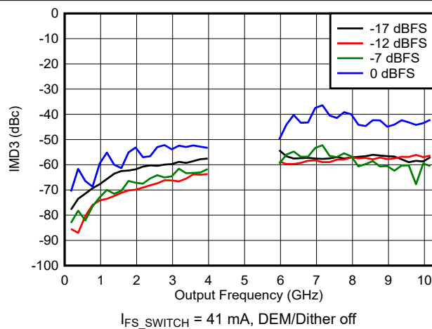
Figure 6-123. IMD3 vs Frequency and Digital Amplitude in DES2X Modes
