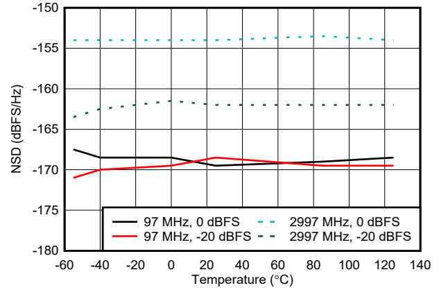
Figure 6-83. NSD vs Temperature
