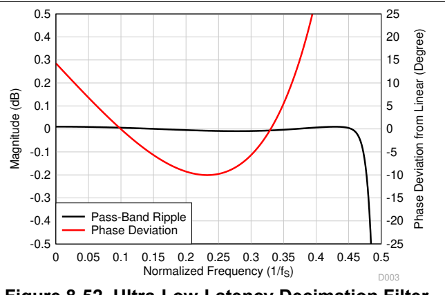
Figure 8-52. Ultra-Low-Latency Decimation Filter Pass-Band Ripple and Phase Deviation
