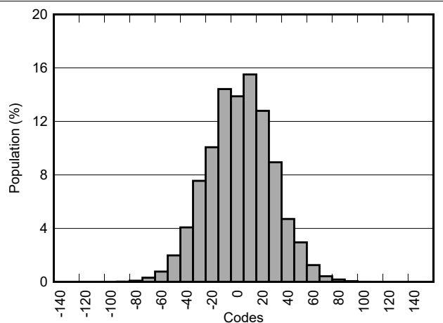
OSR = 64 (262,144 samples)
