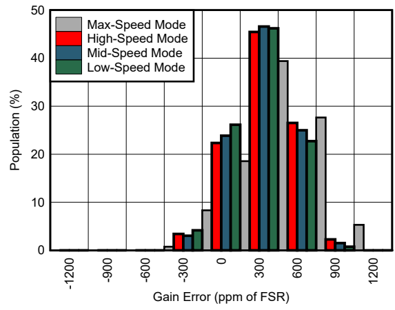
Figure 5-41. Gain Error Histograms
