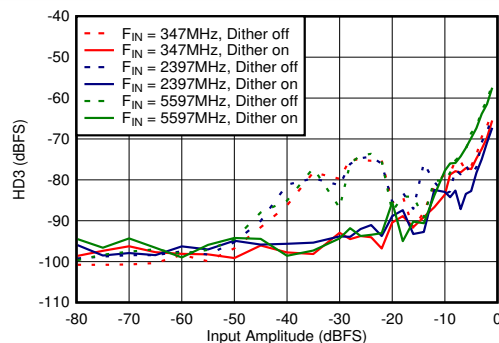
Figure 5-66. DES Mode: HD3 vs Input Amplitude and Dither
