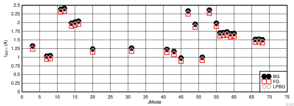
Figure 5-116. Dual Channel Mode: I_{VA11} vs JMODE at 5.2GSPS
