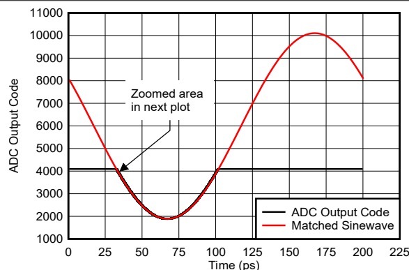
Figure 5-150. Sinewave Overdrive Recovery
