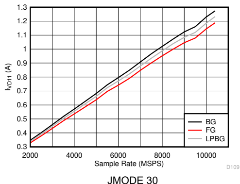
Figure 5-127. DES Mode: I_{VD11} vs Sample Rate
