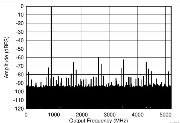
Figure 5-6. DES Mode: Single Tone FFT at 897MHz
