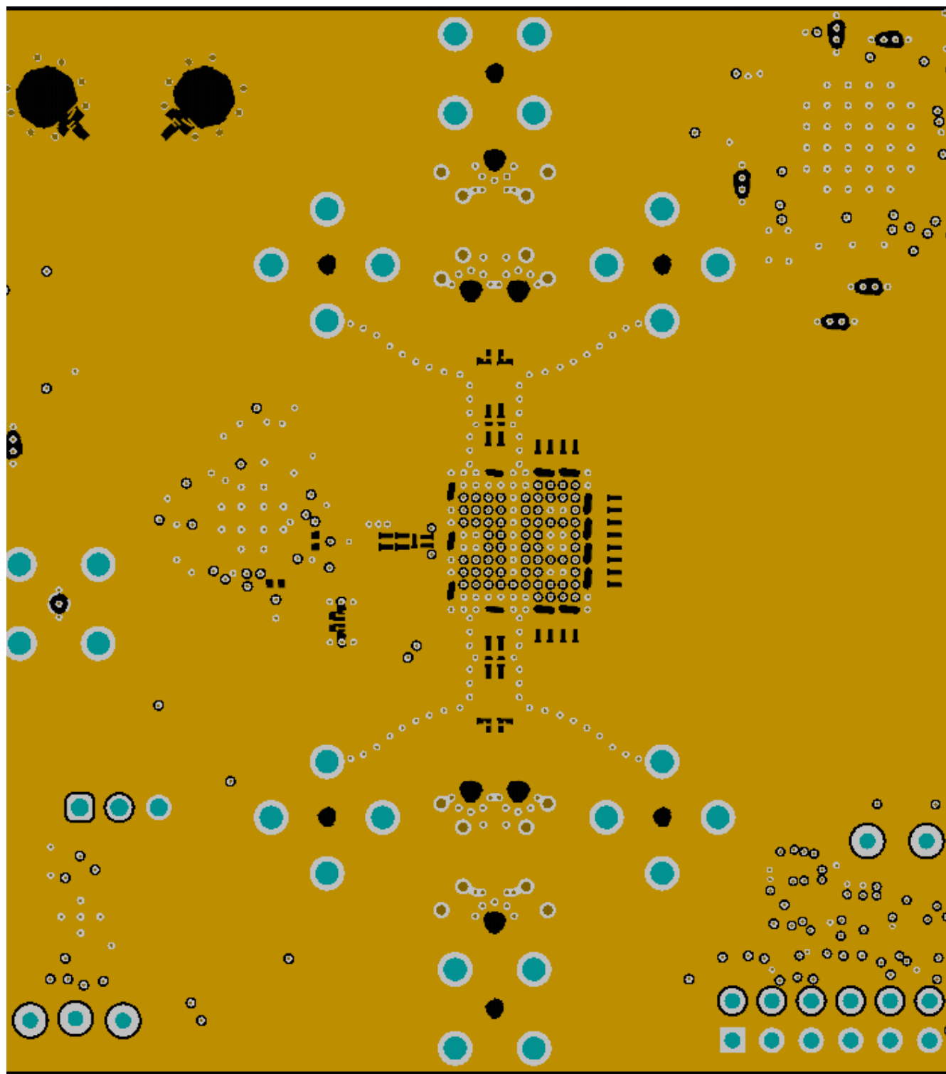
Figure 7-8. GND1 Cutouts to Optimize Impedance of Component Pads
