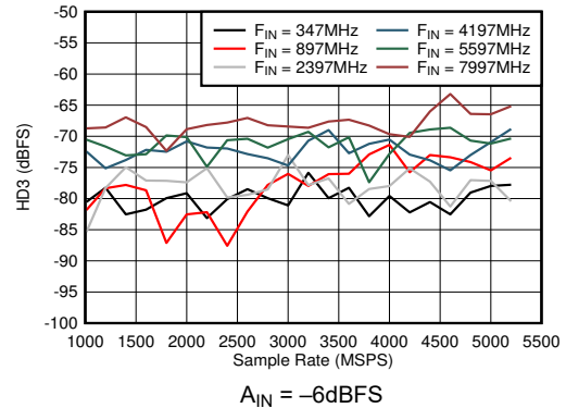
Figure 5-56. Dual Channel Mode: HD3 vs Sample Rate and Input Frequency
