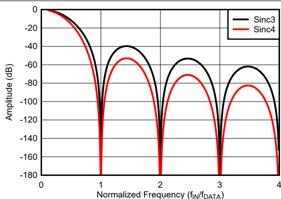
Figure 7-24. Sinc3 and Sinc4 Frequency Response (OSR = 32)
