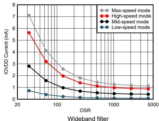
Figure 5-92. IOVDD Current vs Oversampling Ratio
