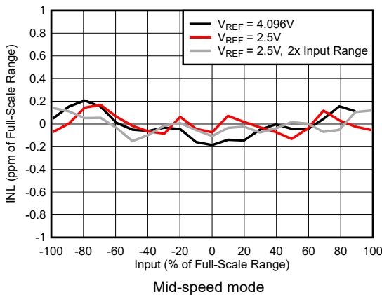
Figure 5-65. INL Error vs Input Voltage
