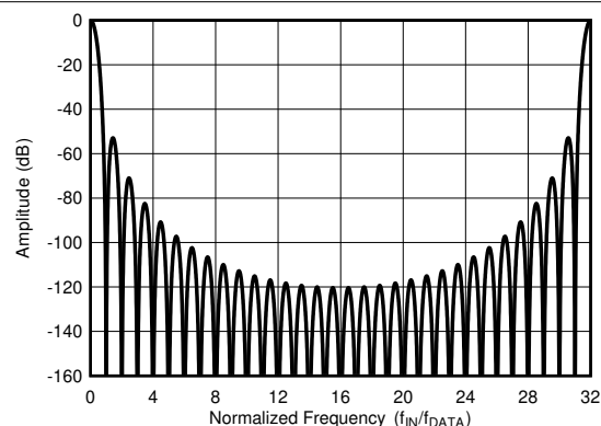
Figure 7-25. Sinc4 Frequency Response to f_{\text{MOD}} (OSR = 32)
