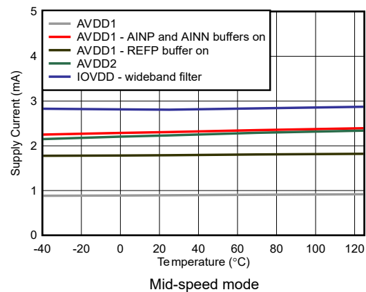
Figure 5-90. Power-Supply Current vs Temperature
