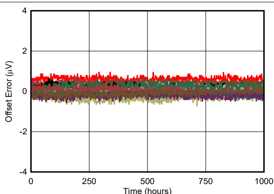
Figure 5-51. Long-Term Offset Drift
