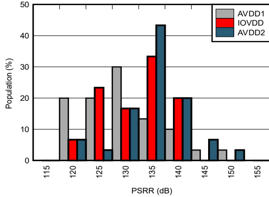
Figure 5-85. DC PSRR Distribution
