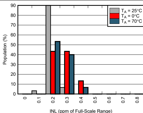
Figure 5-69. INL Distributions
