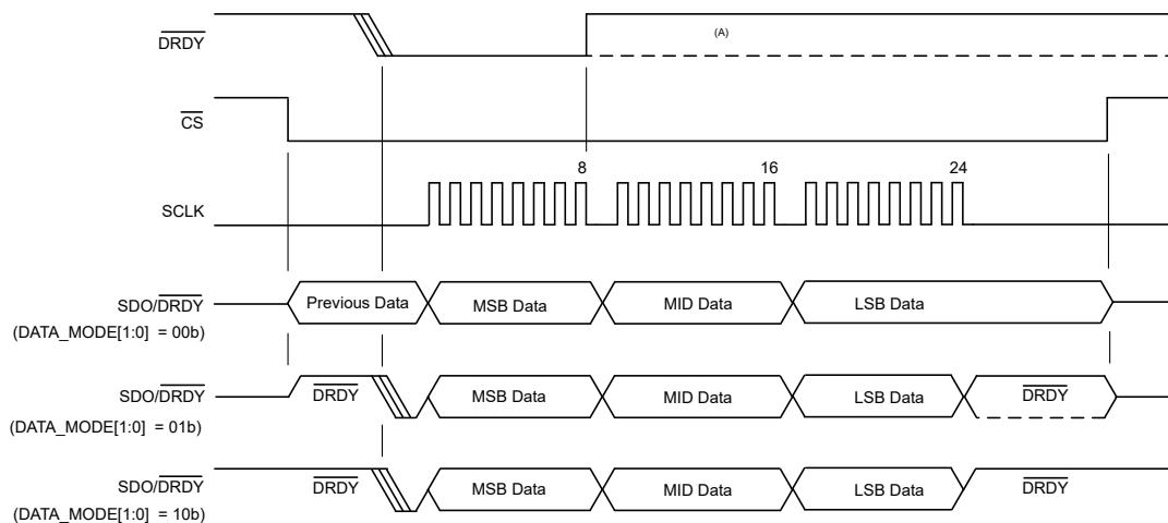
Figure 7-41. SDO/ \overline{\text{DRDY}} and \overline{\text{DRDY}} Function
