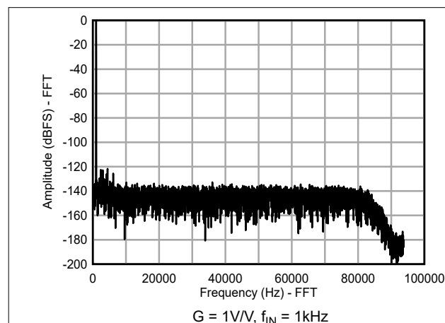
Figure 9-5. Wideband Filter Performance
