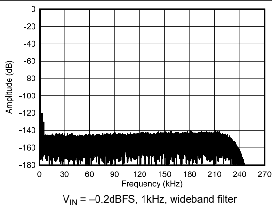
Figure 5-12. Max-Speed Mode, Full-Scale FFT
