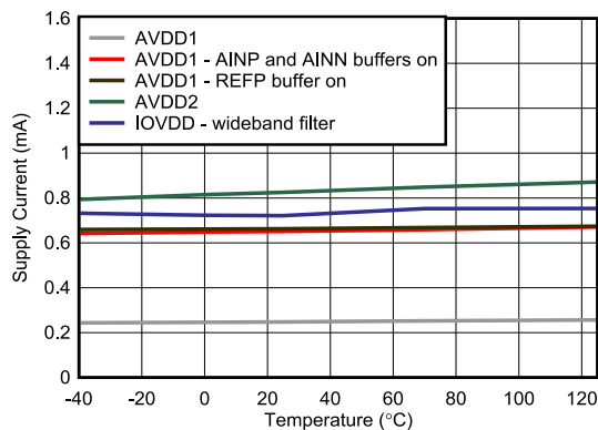
Figure 5-91. Power-Supply Current vs Temperature
