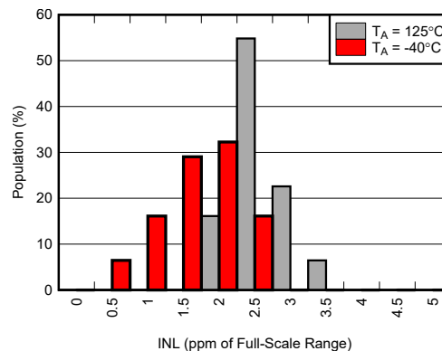
Figure 5-68. INL Distributions
