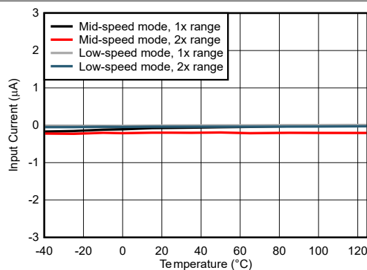
Figure 5-46. Input Current vs Temperature
