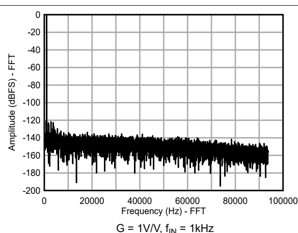
Figure 9-6. Sinc4 Filter Performance
