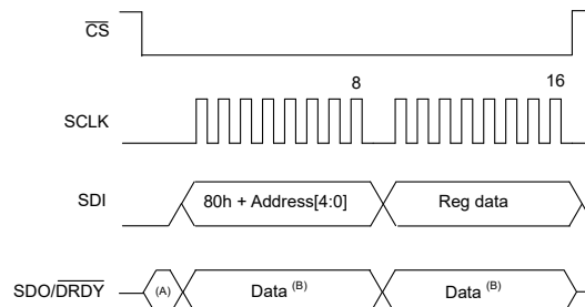
Figure 7-37. Write Register Data, Minimum 16-Bit Frame Size
