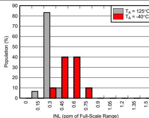
Figure 5-70. INL Distributions
