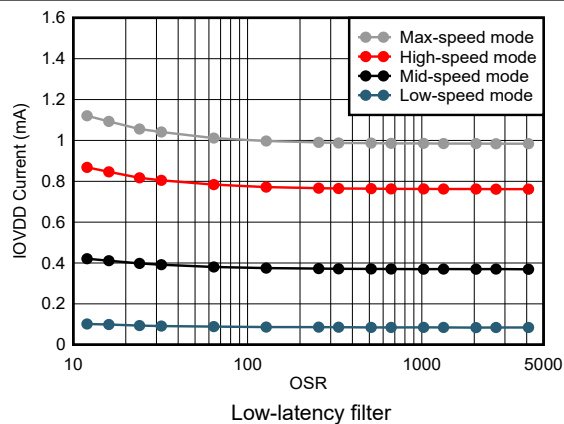
Figure 5-93. IOVDD Current vs Oversampling Ratio
