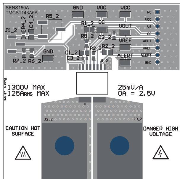
Figure 5-10. TMCS1143EVM, 60 Percent of EVM Plane
