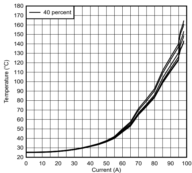
Figure 5-9. TMCS1143EVM Thermal Response Curves for 6 Devices, 40 Percent of EVM Plane
