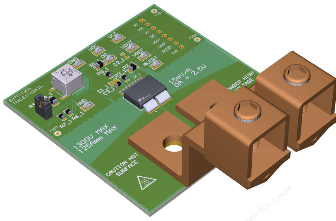
Figure 2-2. TMCS1143EVM Single Panel
