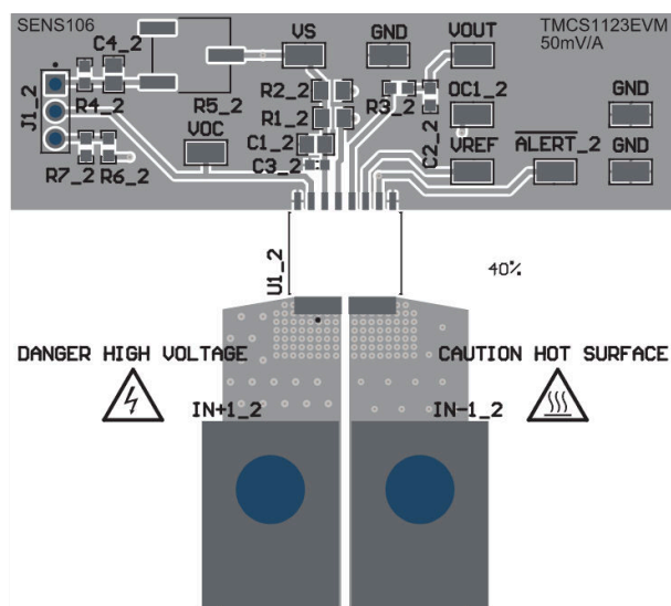
Figure 5-1. TMCS1123EVM, 40 Percent of EVM Plane
