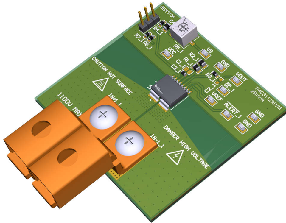
Figure 2-1. TMCS1123EVM Single Panel
