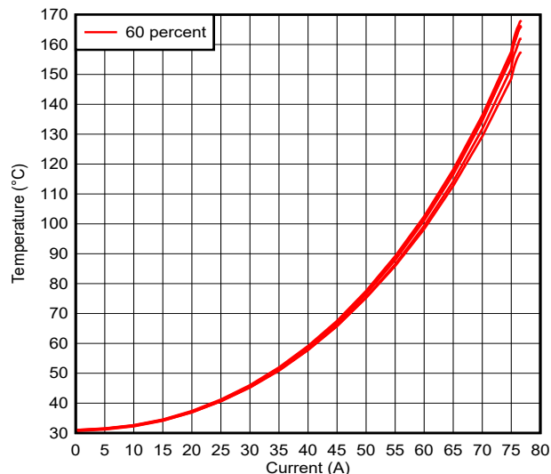
Figure 5-4. TMCS1123EVM Thermal Response Curves for 5 Devices, 60 Percent of EVM Plane
