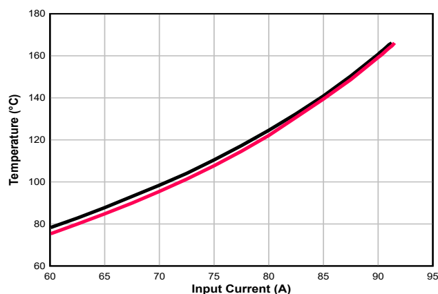
Figure 2-3. TMCS1123EVM Thermal Response Curves for 2 Sample Devices, 3oz Copper, >60 Amperes
