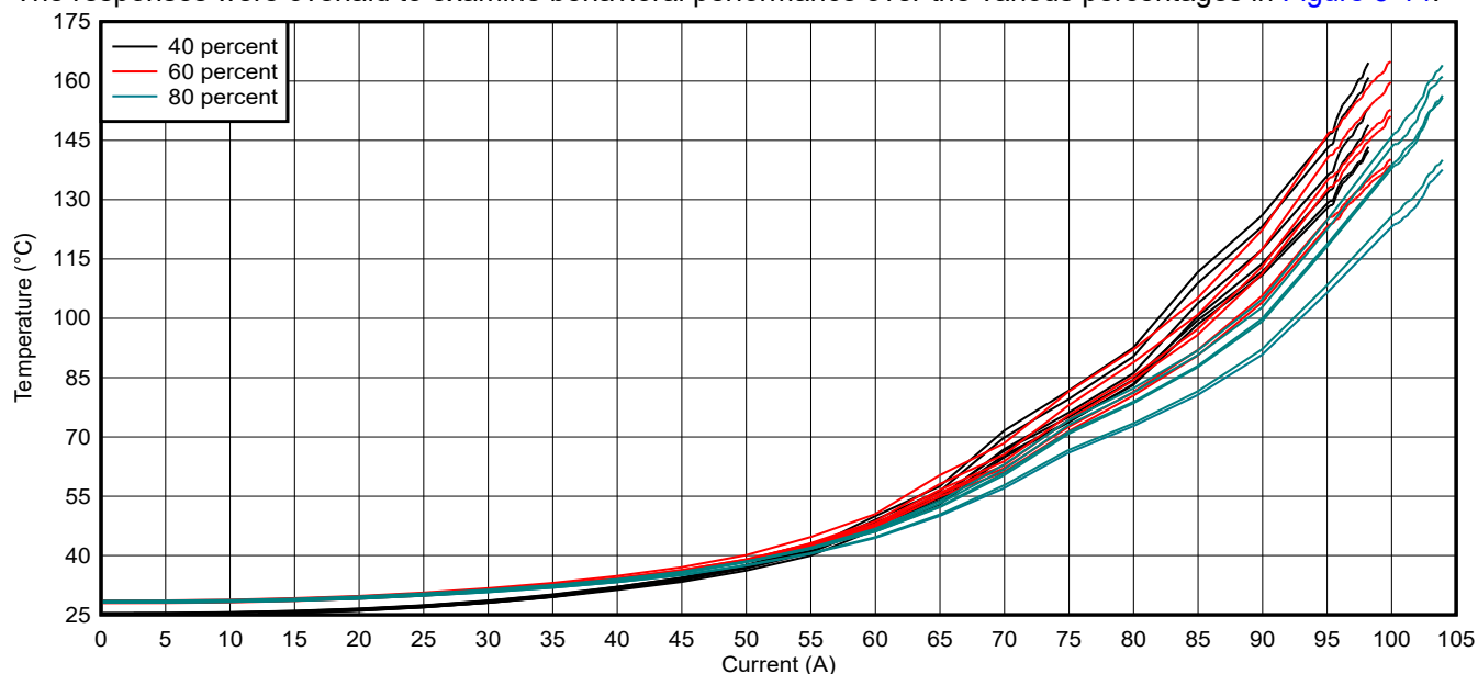
Figure 5-14. TMCS1143EVM Thermal Response Curves for all Copper Sizes
