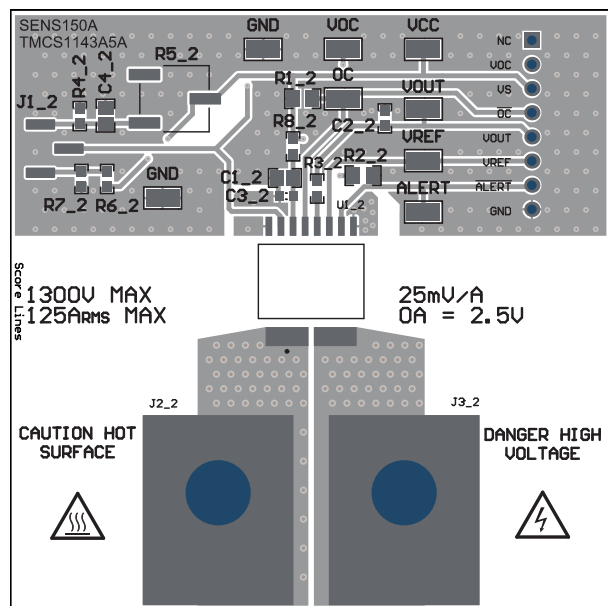
Figure 5-8. TMCS1143EVM, 40 Percent of EVM Plane
