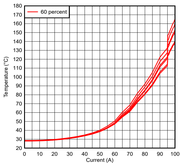
Figure 5-11. TMCS1143EVM Thermal Response Curves for 6 Devices, 60 Percent of EVM Plane
