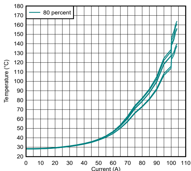
Figure 5-13. TMCS1143EVM Thermal Response Curves for 6 Devices, 80 Percent of EVM Plane
