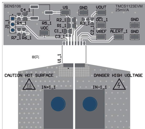
Figure 5-5. TMCS1123EVM, 80 Percent of EVM Plane
