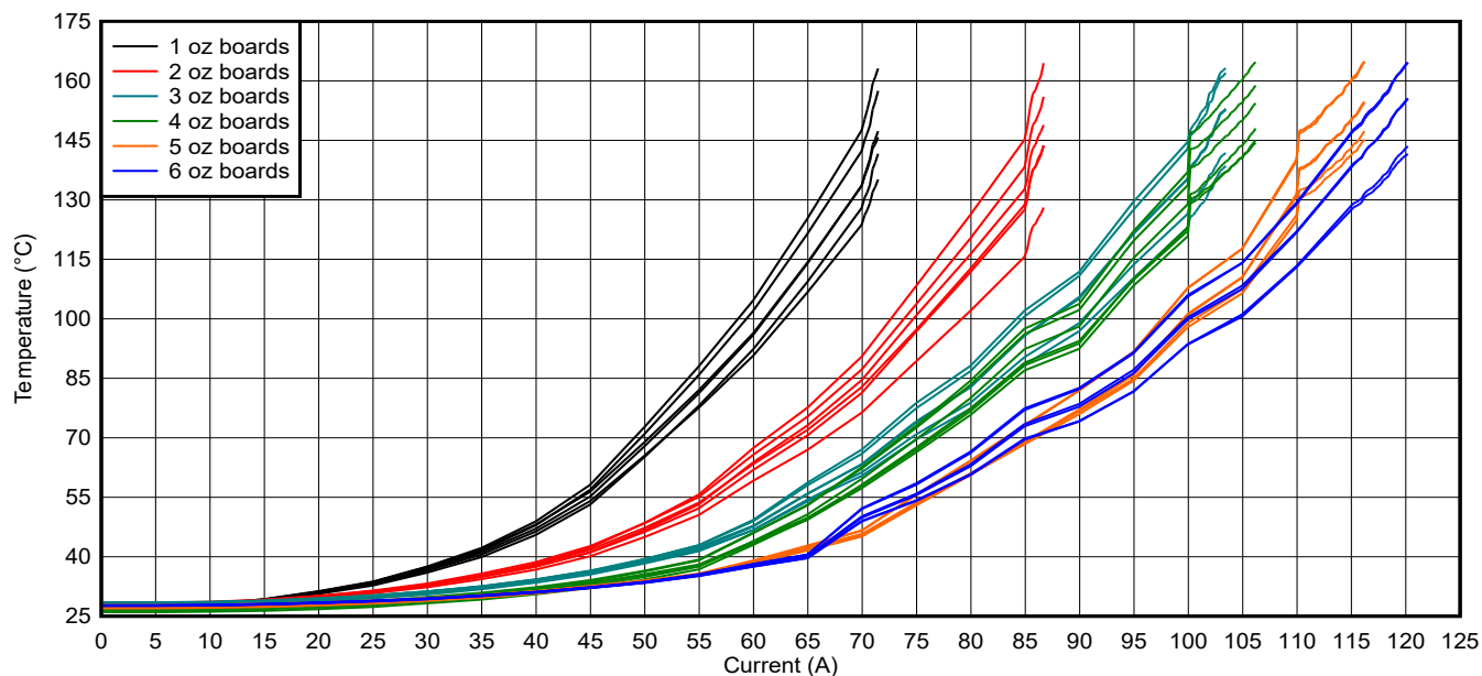
Figure 4-4. TMCS1143EVM Thermal Response Curves for all Copper Weights
