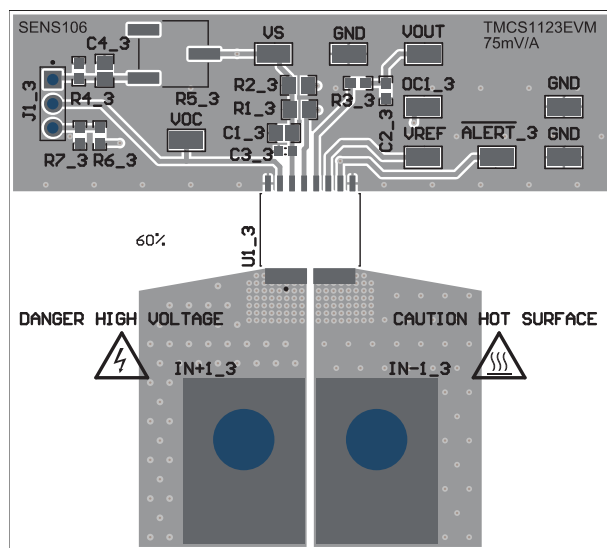
Figure 5-3. TMCS1123EVM, 60 Percent of EVM Plane
