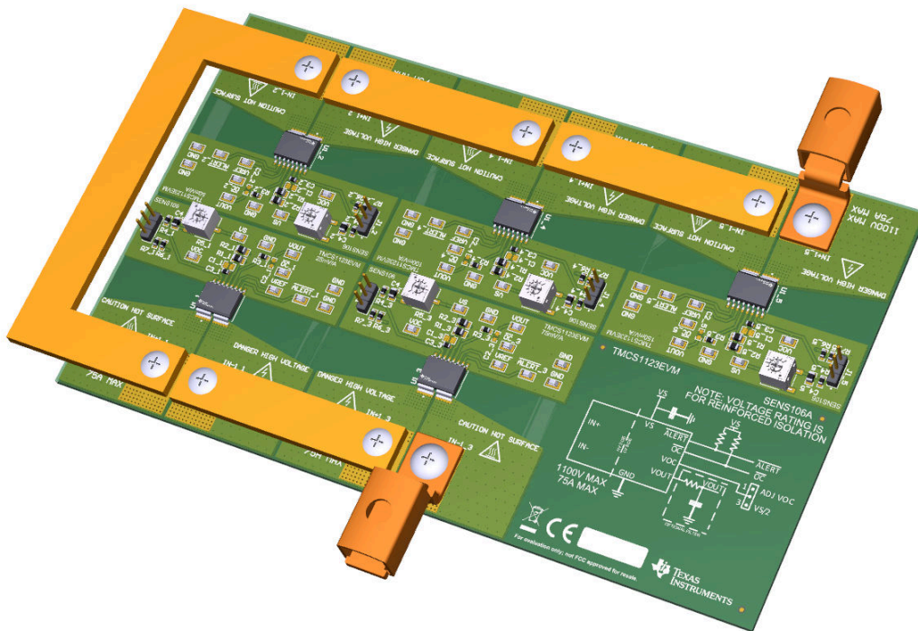
Figure 3-1. TMCS1123EVM, Bus Bar Configuration
