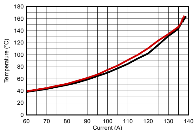
Figure 2-6. TMCS1143EVM Thermal Response Curves for 2 Devices, 4oz Copper, >60 Amperes
