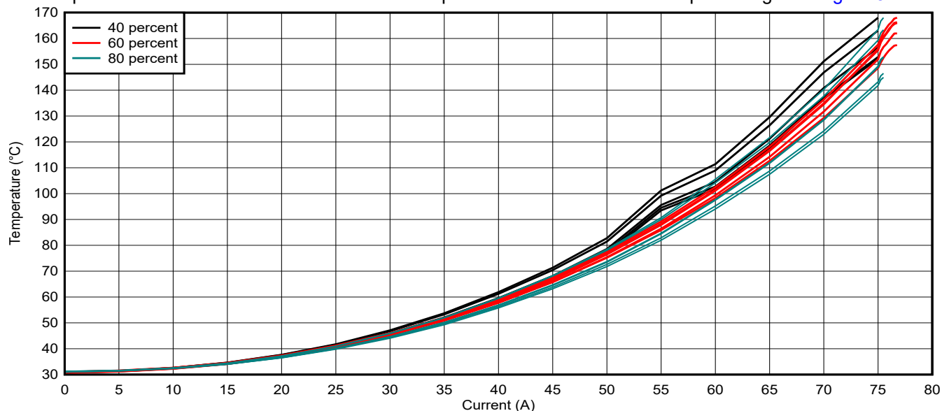
Figure 5-7. TMCS1123EVM Thermal Response Curves for all Copper Sizes
