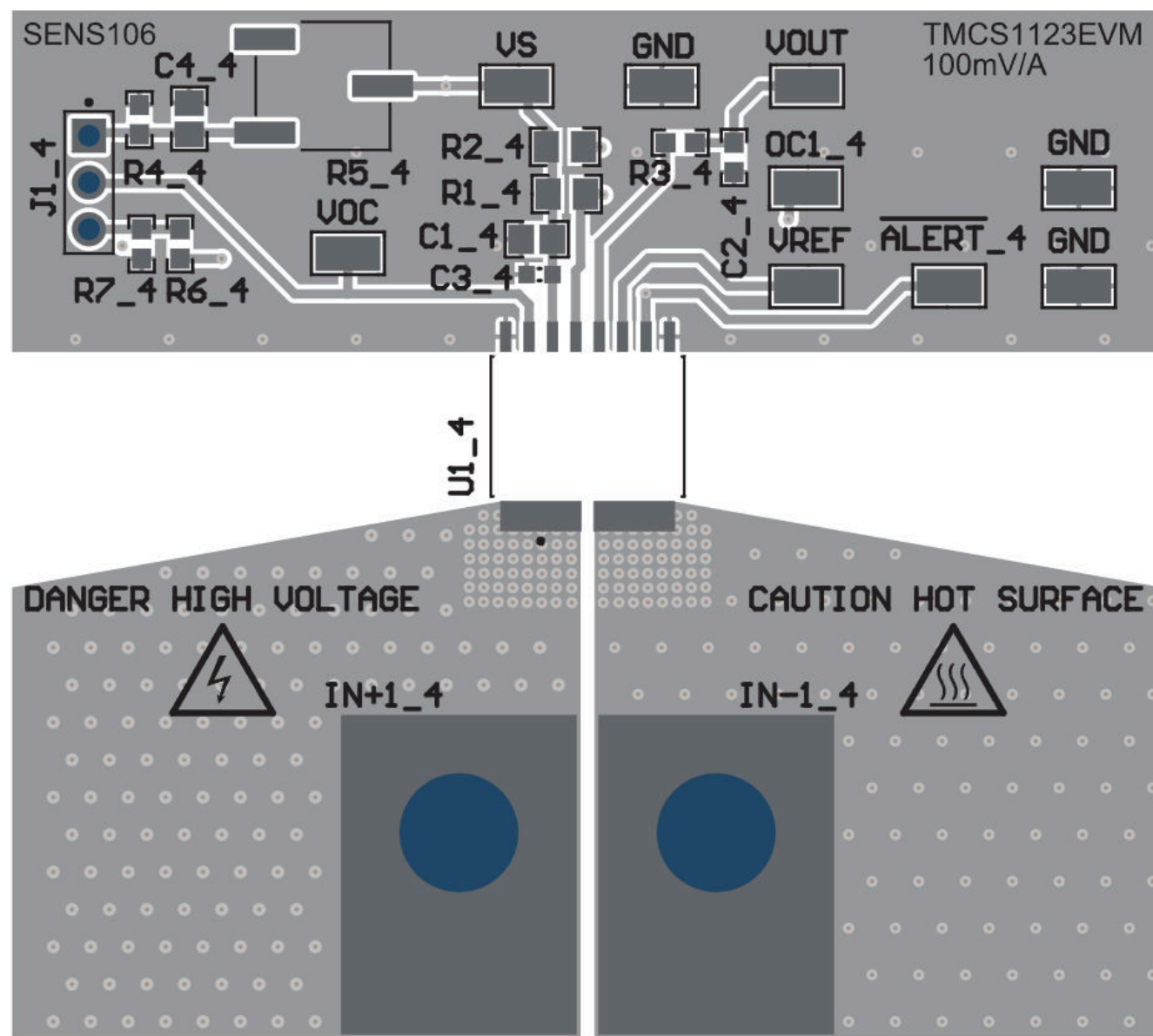
Figure 4-1. TMCS1123EVM Portion
