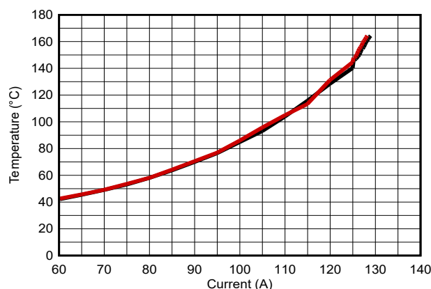
Figure 2-5. TMCS1143EVM Thermal Response Curves for 2 Sample Devices, 3oz Copper, >60 Amperes
