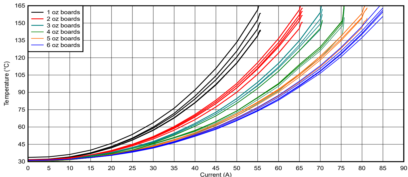
Figure 4-2. TMCS1123EVM Thermal Response Curves for all Copper Weights
