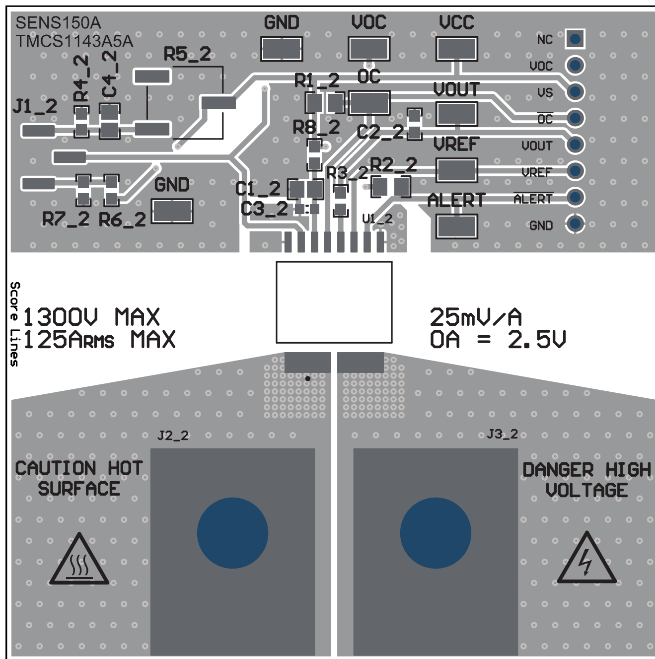
Figure 4-3. TMCS1143EVM Portion
