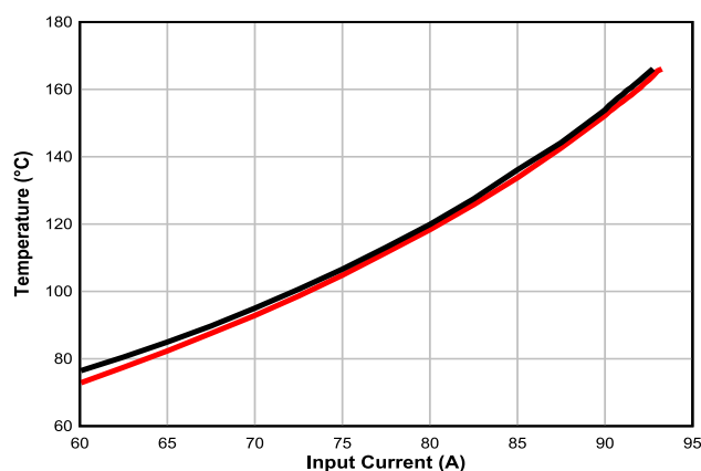
Figure 2-4. TMCS1123EVM Thermal Response Curves for 2 Devices, 4oz Copper, >60 Amperes
