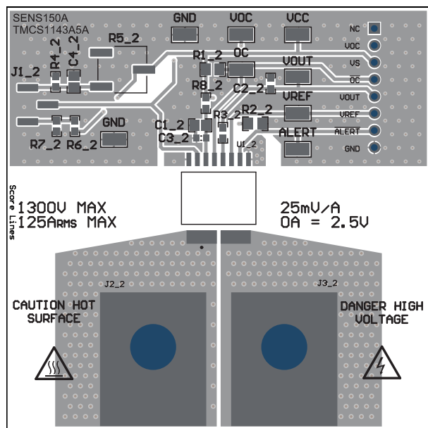
Figure 5-12. TMCS1143EVM, 80 Percent of EVM Plane
