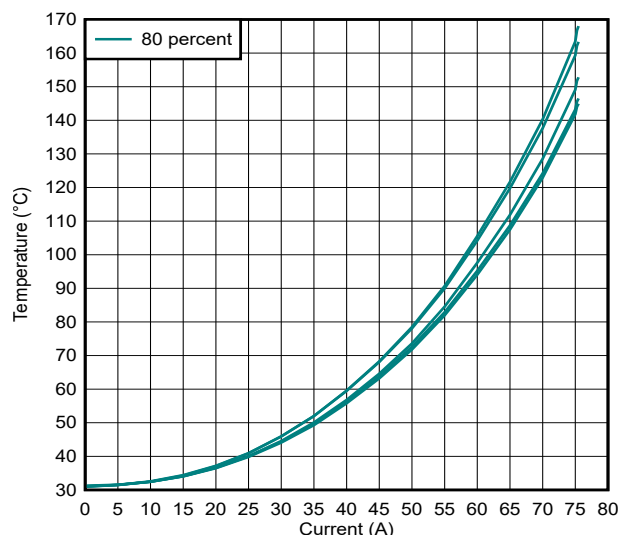
Figure 5-6. TMCS1123EVM Thermal Response Curves for 5 Devices, 80 Percent of EVM Plane
