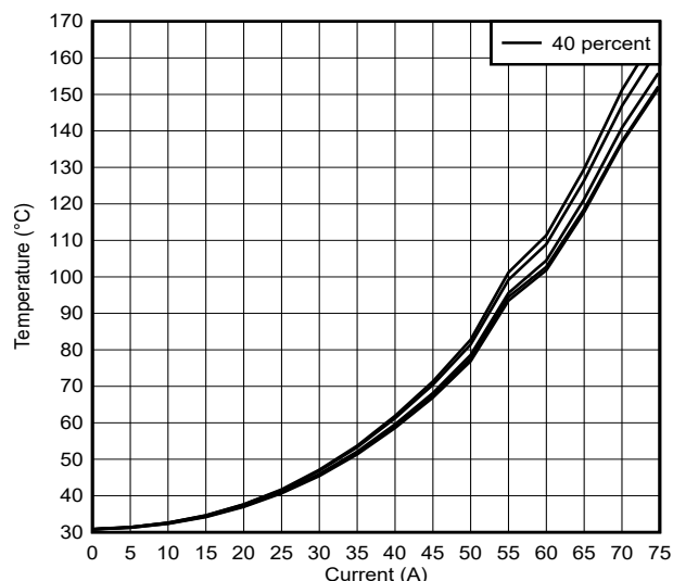
Figure 5-2. TMCS1123EVM Thermal Response Curves for 5 Devices, 40 Percent of EVM Plane
