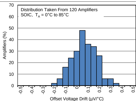
OPA192ID and OPA2192ID
