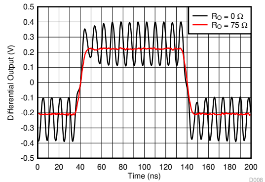
Figure 6-8. Step Response Into Capacitive Load
