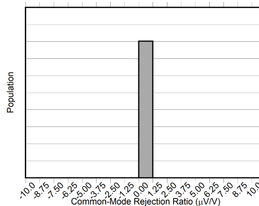
Figure 5-5. CMRR Production Distribution
