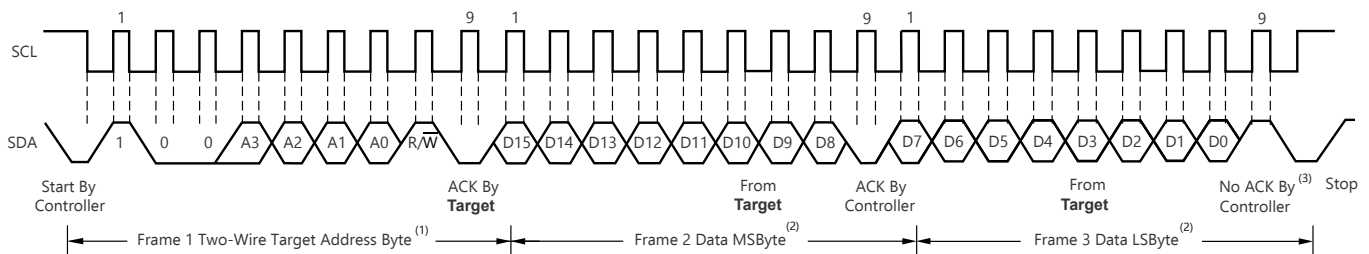
Figure 6-3. Timing Diagram for Write Word Format
