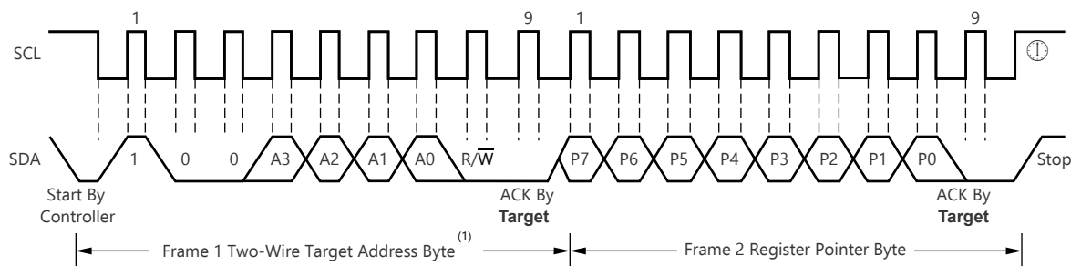
Figure 6-5. Typical Register Pointer Set
