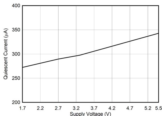
Figure 5-19. Quiescent Current vs Supply Voltage
