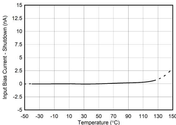
Figure 5-17. Input Bias Current vs Temperature (Shutdown)
