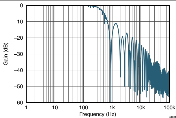
Figure 5-2. Frequency Response
