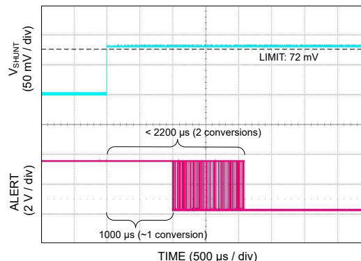
Figure 7-4. Alert Response ( t_{CT} = 1.1ms )
