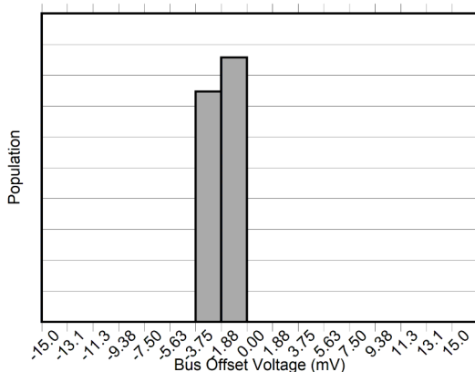
Figure 5-10. Bus Offset Voltage ( V_{IN-} ) Production Distribution
