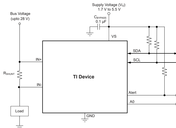
Figure 7-2. Typical High-Side Sensing Circuit Configuration, INA234
