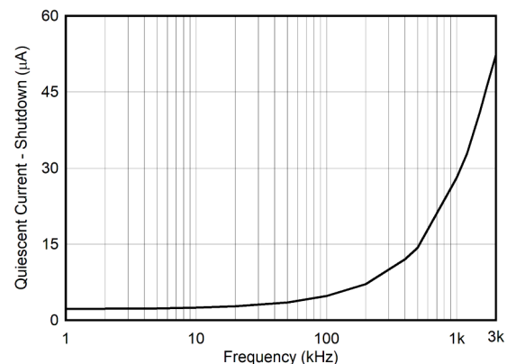
Figure 5-23. Quiescent Current - Shutdown vs SCL Frequency
