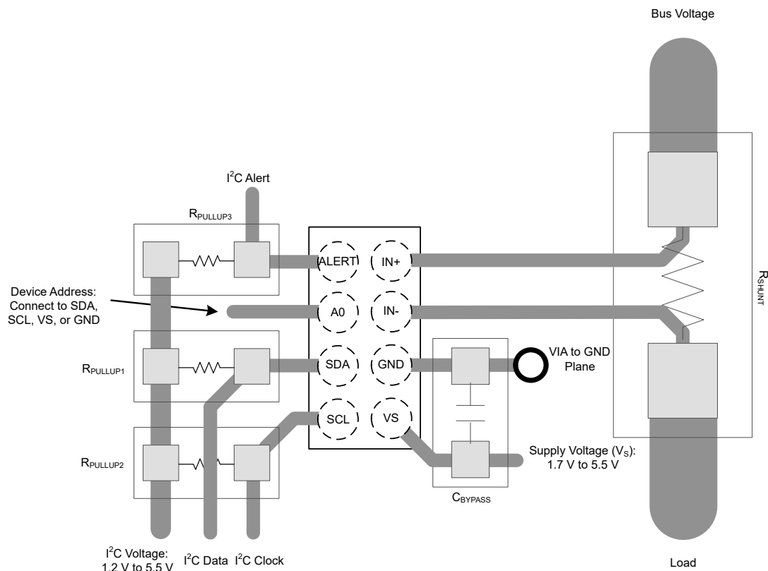
Figure 7-5. INA234 Layout Example DSBGA (High Side)
