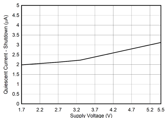
Figure 5-20. Quiescent Current - Shutdown vs Supply Voltage
