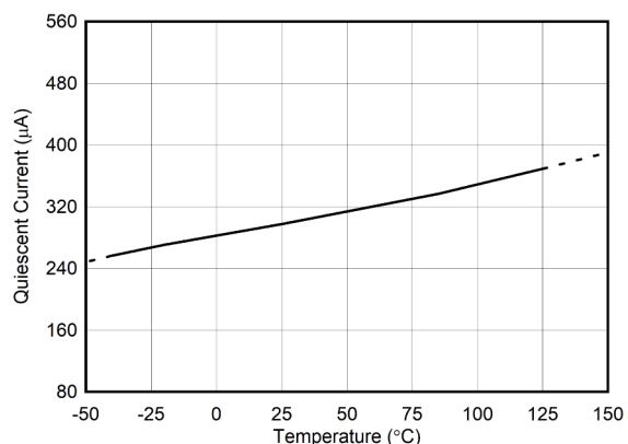
Figure 5-18. Quiescent Current vs Temperature
