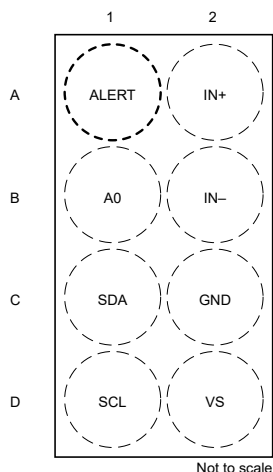
Figure 4-1. YBJ Package 8-Bump DSBGA (Top View)
