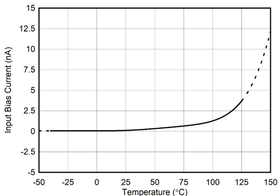
Figure 5-16. Input Bias Current vs Temperature
