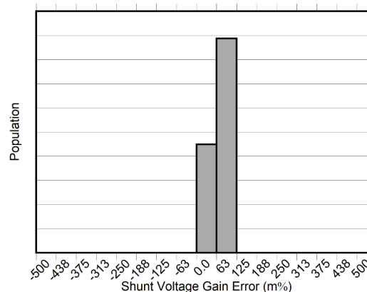
Figure 5-7. Shunt Voltage Gain Error Production Distribution
