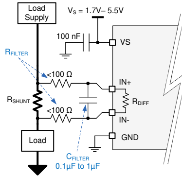
Figure 7-1. Input Filtering
