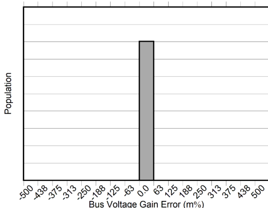
Figure 5-12. Bus Voltage ( V_{IN-} ) Gain Error Production Distribution
