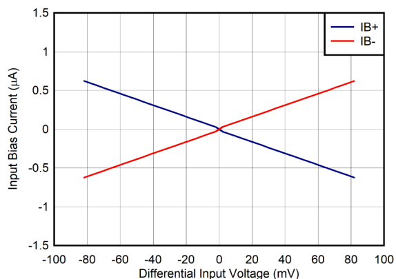
Figure 5-14. Input Bias Current vs Differential Voltage
