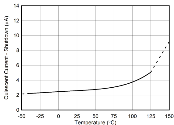
Figure 5-21. Quiescent Current - Shutdown vs Temperature
