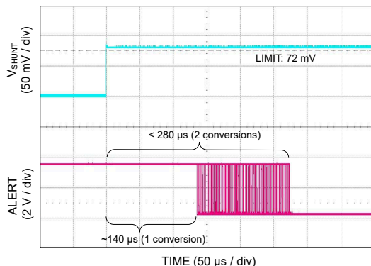
Figure 7-3. Alert Response ( t_{CT} = 140\mu s )
