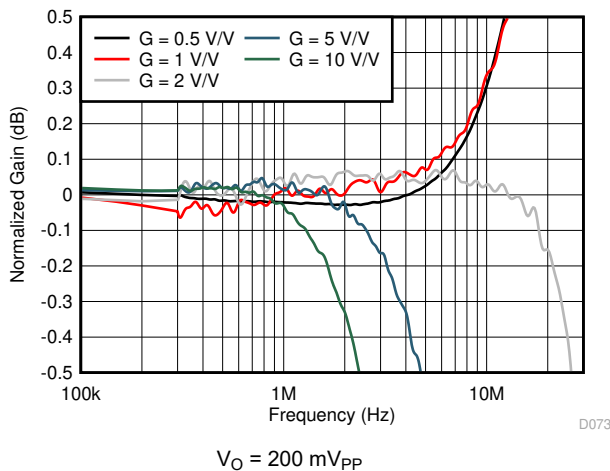
Figure 7-19. Gain Flatness vs Frequency
