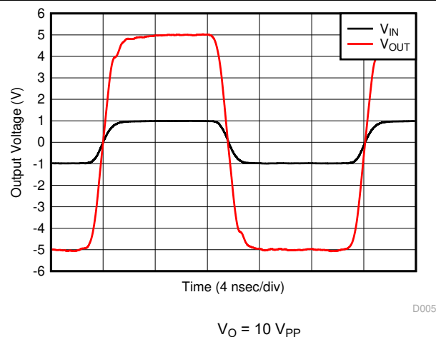
Figure 8-23. G = 5 V/V Pulse Response V_O = 10 V PP
