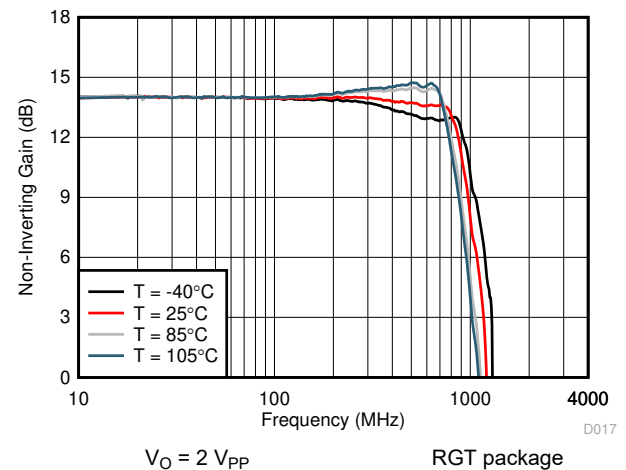
Figure 8-6. Frequency Response vs Temperature
