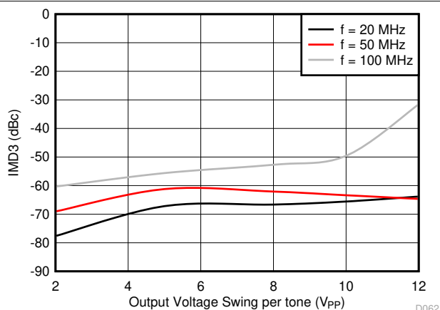
Figure 8-20. IMD3 vs Output Voltage Swing \pm 100 -kHz frequency spacing
