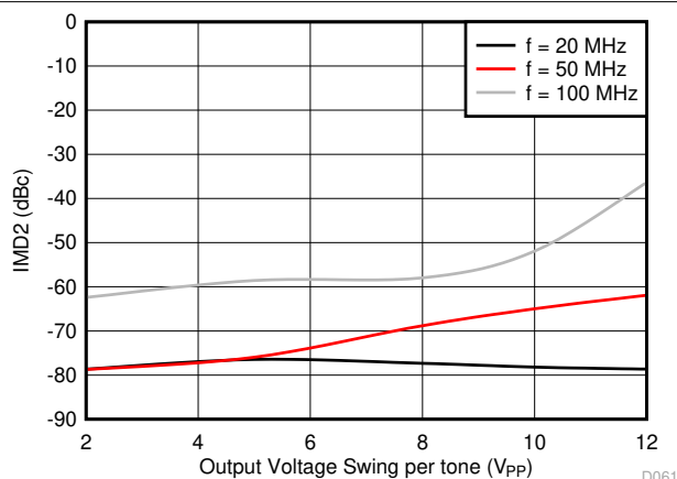
Figure 8-19. IMD2 vs Output Voltage Swing \pm 100 -kHz frequency spacing
