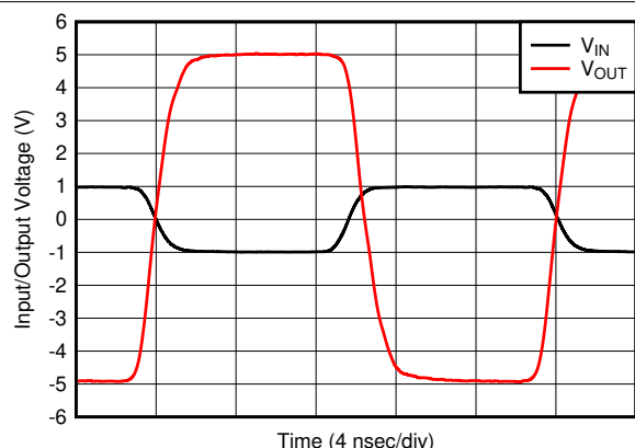
Figure 8-25. G = -5 V/V Pulse Response
