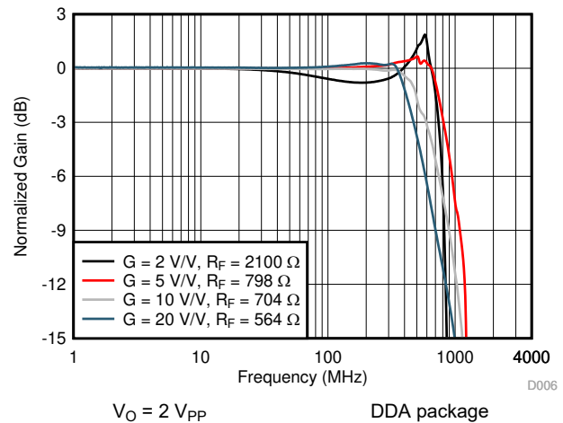
Figure 8-2. Noninverting Small-Signal Frequency Response
