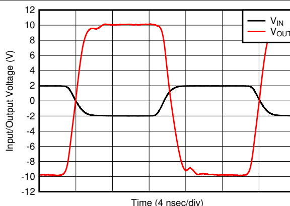
Figure 8-26. G = -5 V/V Pulse Response
