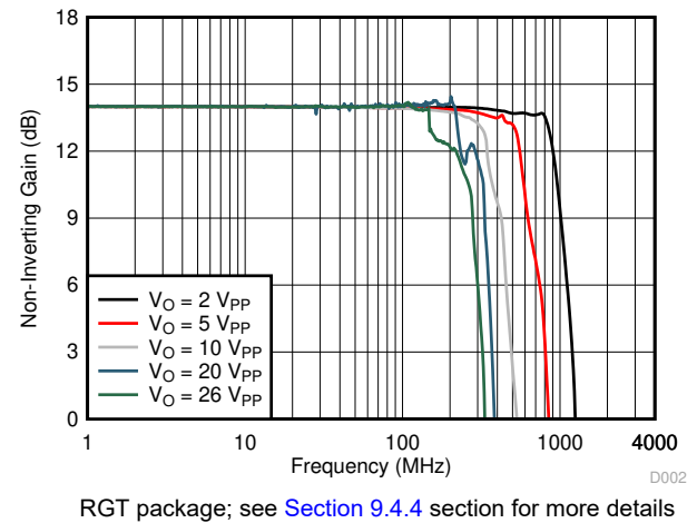
Figure 8-4. Frequency Response vs Output Swing
