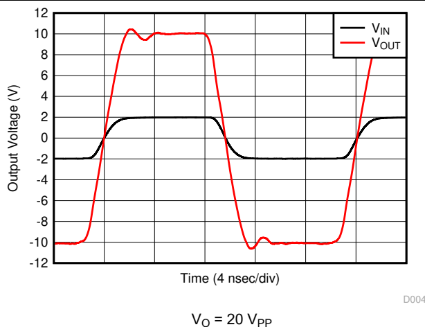
Figure 8-24. G = 5 V/V Pulse Response V_O = 20 V PP
