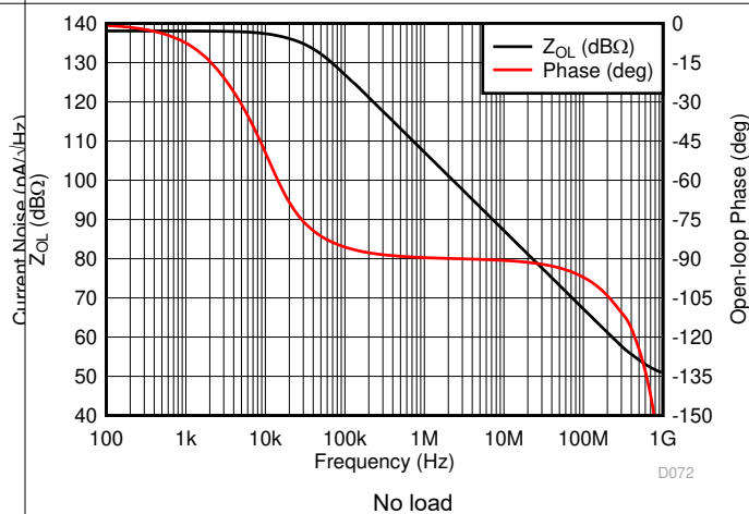
Figure 8-22. Open-Loop Transimpedance Gain and Phase vs Frequency No load
