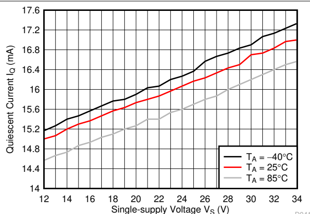
Figure 8-30. Quiescent Current vs Supply Voltage
