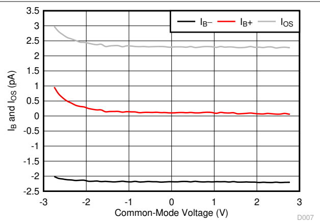
Figure 5-2. I_B and I_{OS} vs Common-Mode Voltage
