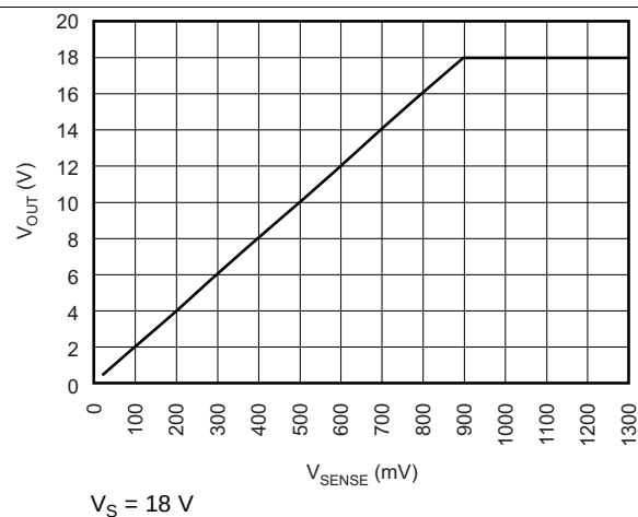
Figure 3. Gain Plot
