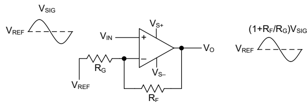
Figure 7-1. Noninverting Amplifier
