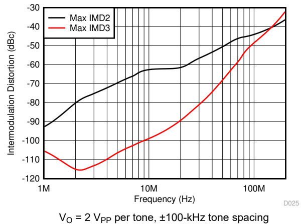
Figure 6-16. Inter Modulation Distortion vs Frequency
