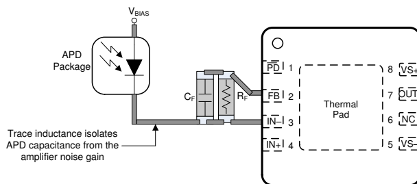
Figure 8-10. Non-Ideal TIA Layout
