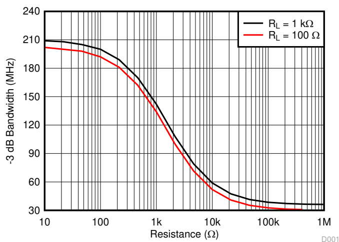
Figure 8-2. Small-Signal Bandwidth versus Bandwidth Adjustment Resistance
