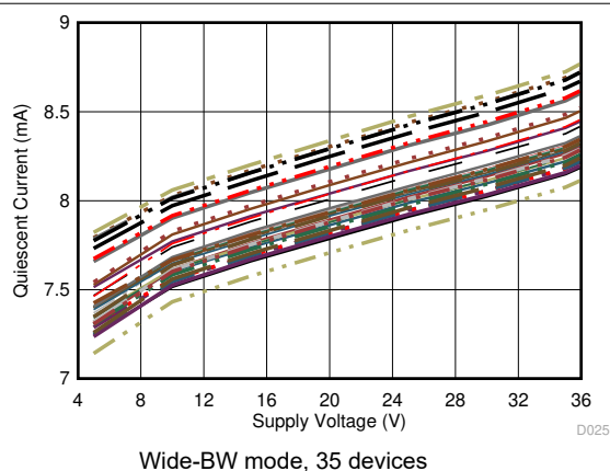
Figure 7-30. Quiescent Current vs Supply Voltage
