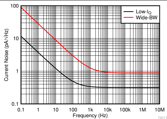
Figure 7-10. Current Noise Density vs Frequency
