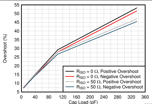
Figure 6-3. Small-Signal Overshoot vs Capacitive Load (10-mV Output Step, G = 1 )
