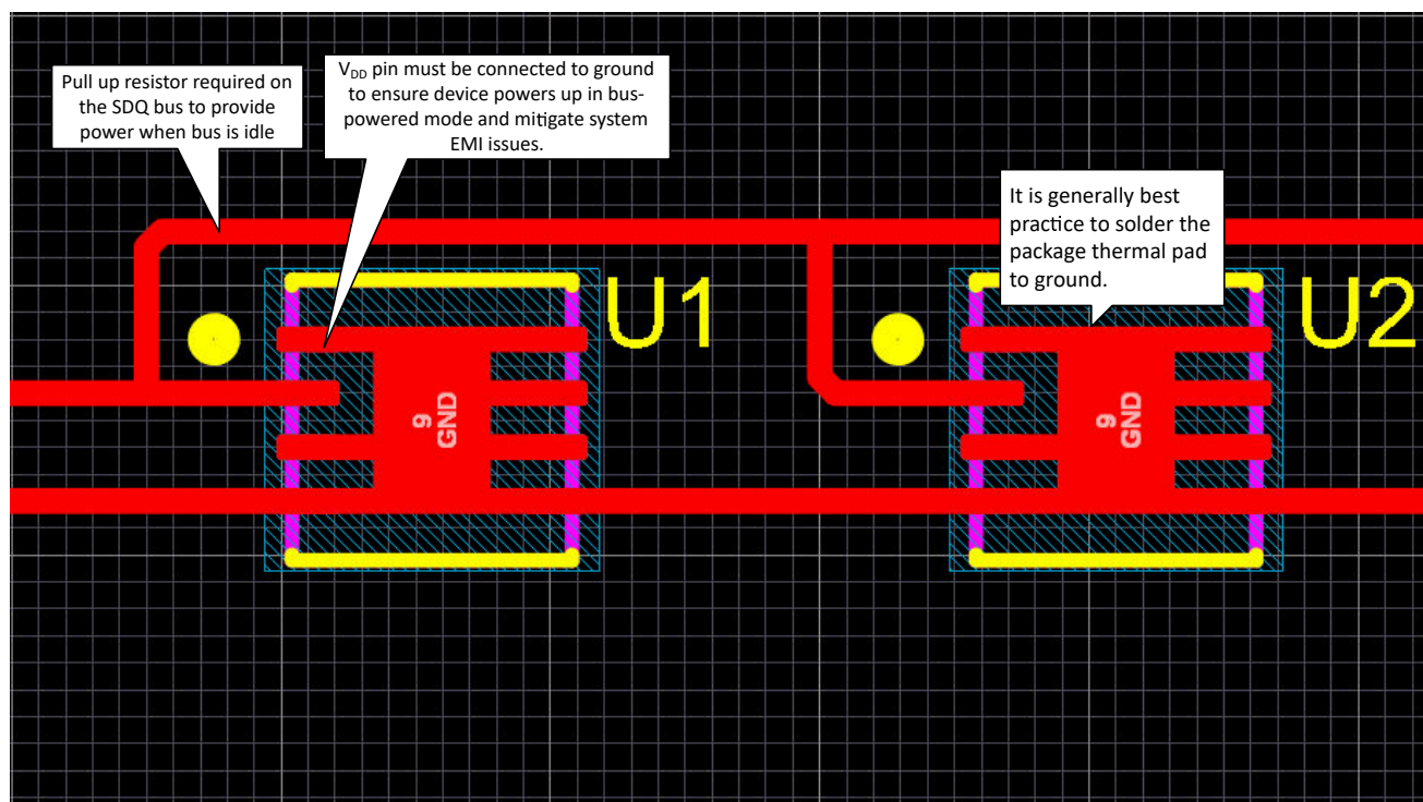
Figure 10-5. Bus Powered Layout Example
