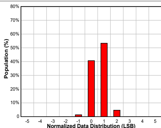
Figure 8-13. Data Distribution With 3-ms Conversion Time and Averaging On in 16-Bit Format
