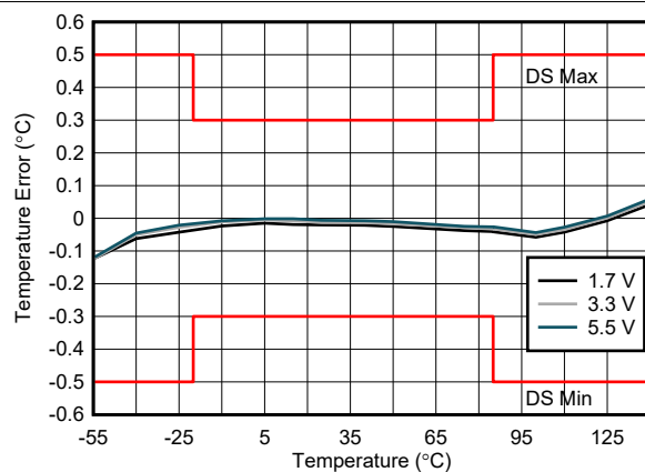
Figure 8-8. Temperature Error vs Temperature (DGK Package)
