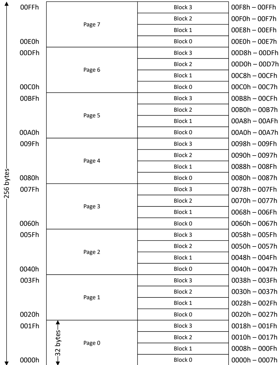
Figure 9-9. Address to EEPROM Page and Block Map
