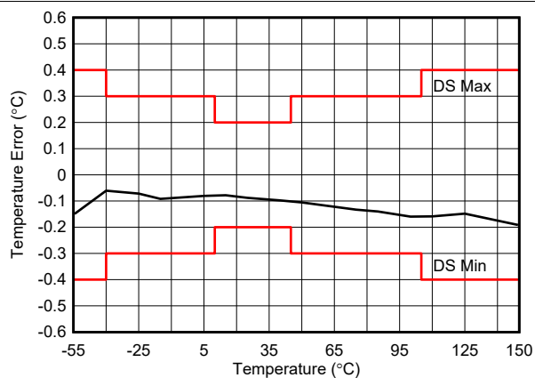
Figure 8-7. Temperature Error vs Temperature (NGR Package)
