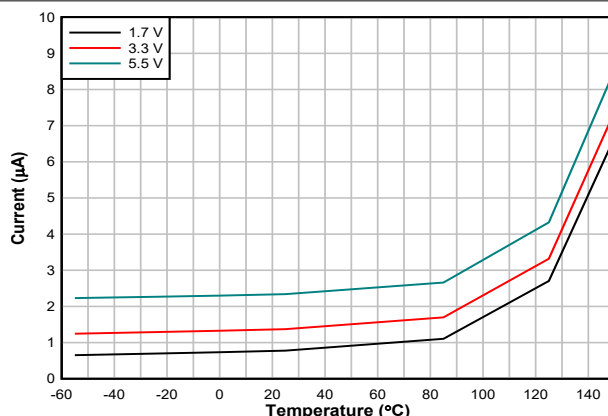
Figure 8-10. Shutdown Current vs Temperature
